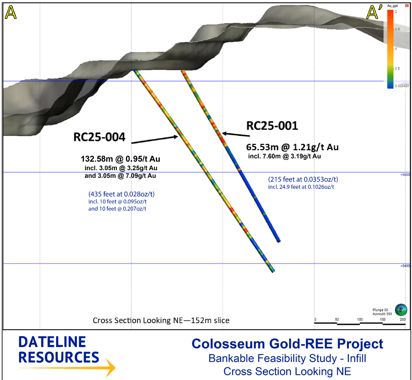
Figure 2: Cross-section of the Colosseum deposit illustrating the existing open pit outline and gold intercepts
