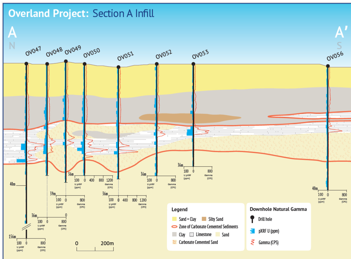
Figure 1: Section A- A' displaying lithology interpretation, natural gamma responses (cps) and pXRF uranium responses (ppm U). In relation to the disclosure of pXRF results, the Company cautions that estimates of uranium elemental abundance from pXRF results should not be considered a proxy for quantitative analysis of a laboratory assay result. Assay results are required to determine the actual widths and grade of the mineralisation. The company uses an Olympus Vanta M Series portable X-ray Fluorescence (pXRF) analyzer to screen Air Core drilling samples for mineralization prior to submitting samples to a commercial laboratory for assay. This provides an initial understanding of the mineralization distribution before sampling, ensuring submitted samples are representative of the targeted mineralization. While pXRF confirms the presence of mineralization, it does not accurately determine elemental concentrations due to limitations such as a small analysis window, uneven distribution, shallow penetration depth, and irregular surfaces. The pXRF results are indicative and the pXRF readings are subject to confirmation by chemical analysis from an independent laboratory.
