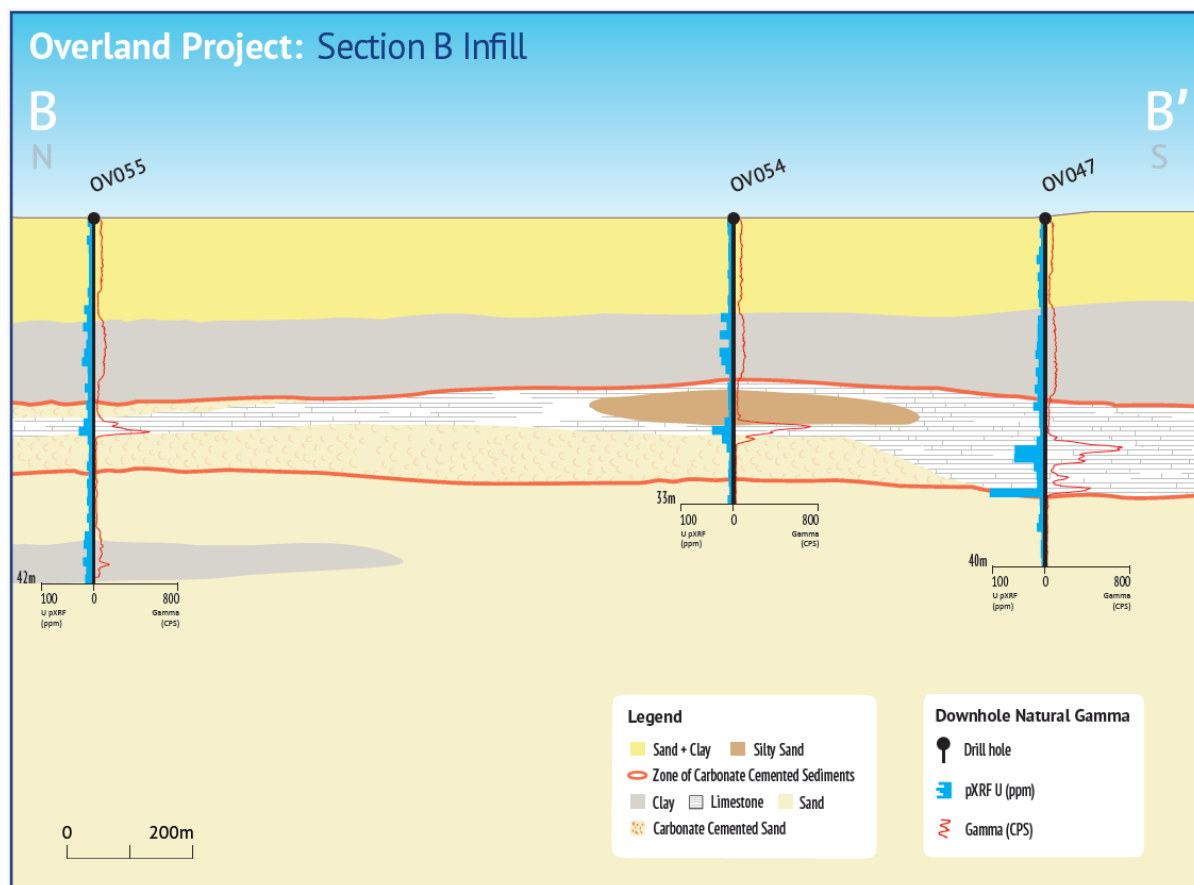
Figure 2: Section B-B' displaying lithology interpretation, natural gamma responses (cps) and pXRF uranium responses (ppm U).
