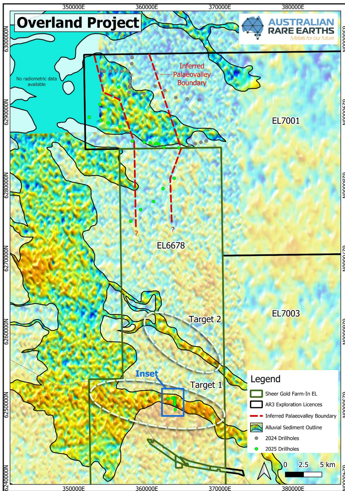
Figure 3: Overland drilling (2024 & 2025) with airborne radiometrics, alluvial sediment channels, and interpreted palaeochannel boundary based on recent drilling. Target 1 follow up drilling shown in inset Figure. Note: The airborne radiometric image and Alluvial Sediment Outline is publicly available data sourced from SARIG ( https://map.sarig.sa.gov.au ) and detailed within the appendices of this report.
