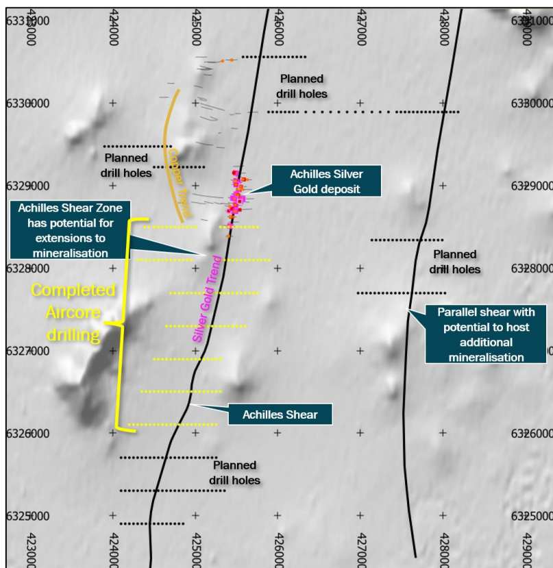
Figure 1: Achilles Shear showing the completed aircore in yellow dots and planned holes in black dots.
