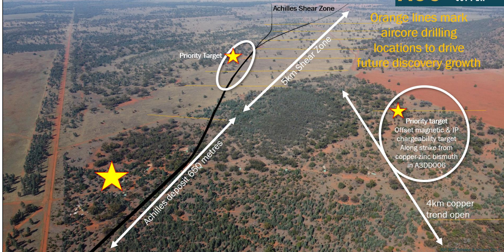
Figure 2: Achilles drone photo, looking south, with annotated locations of the Achilles deposit (foreground) and Achilles shear zone trending south (background). The aircore drilling is underway along the orange lines.
