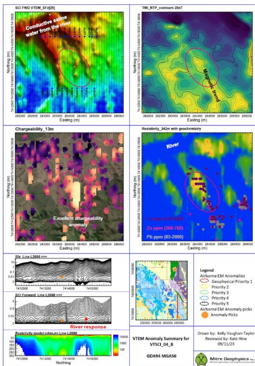
Figure 4: Geophysical summary.
