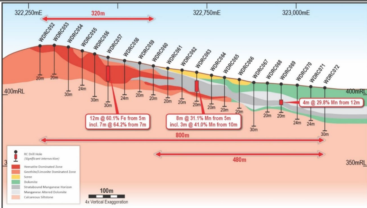
Figure 4. Cross section 7,525,900mN looking to the north showing the location of previously released 1 RC drill holes WDRC057, WDRC063 and WDRC06 (4x Vertical Exaggeration). Note assays pending for other holes.
