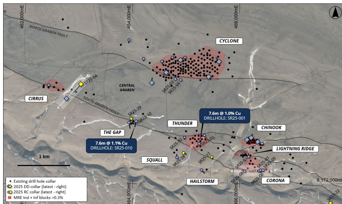
Figure 5: Drill hole locations from the 2025 drilling program (Storm area detail), overlaying deposit MRE outlines and existing drilling overlaying aerial photography. Section views are located on map.
