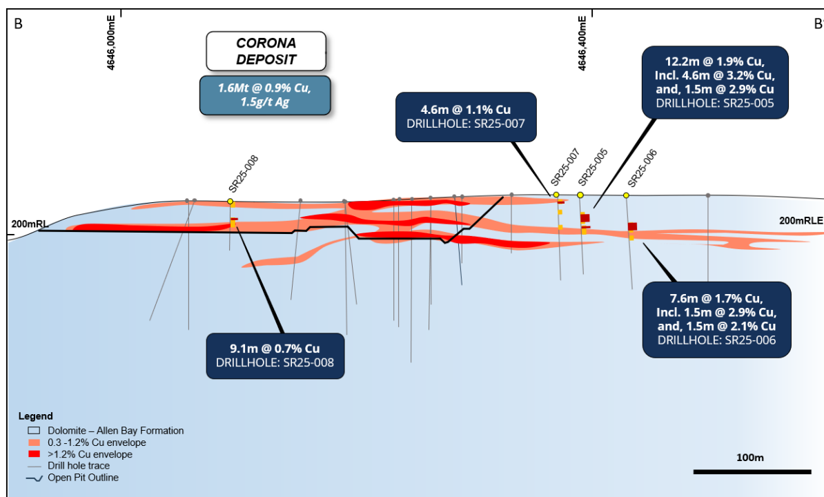
Figure 4: Long-section of the Corona Deposit looking north (+/- 75m) highlighting 2025 drilling, proposed open-pit shell and the MRE copper mineralisation envelope.
