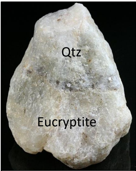
Image depicting the undistinguishable nature of quartz (upper) vs Eucryptite (lower) from the Bikita Pegmatite, Zimbabwe.
