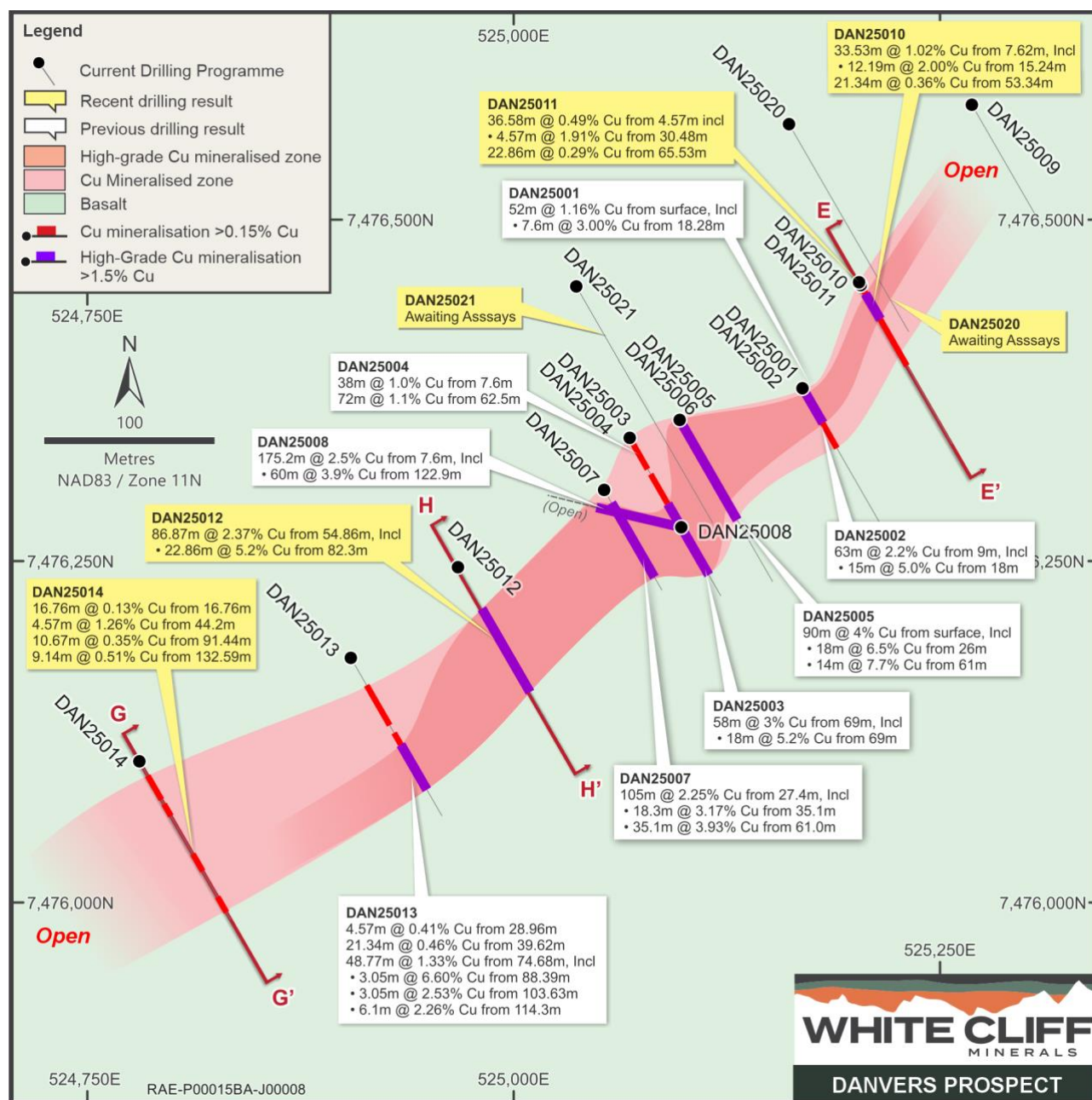
Figure 1 - Plan view of 2025 Spring and Summer RC drillholes at the Danvers Breccia System showing surface projection of intercepted mineralisation. Assay results included in this announcement are shown at E (DAN25010, DAN25011 Figure 3) and G (DAN25014, Figure 2).
