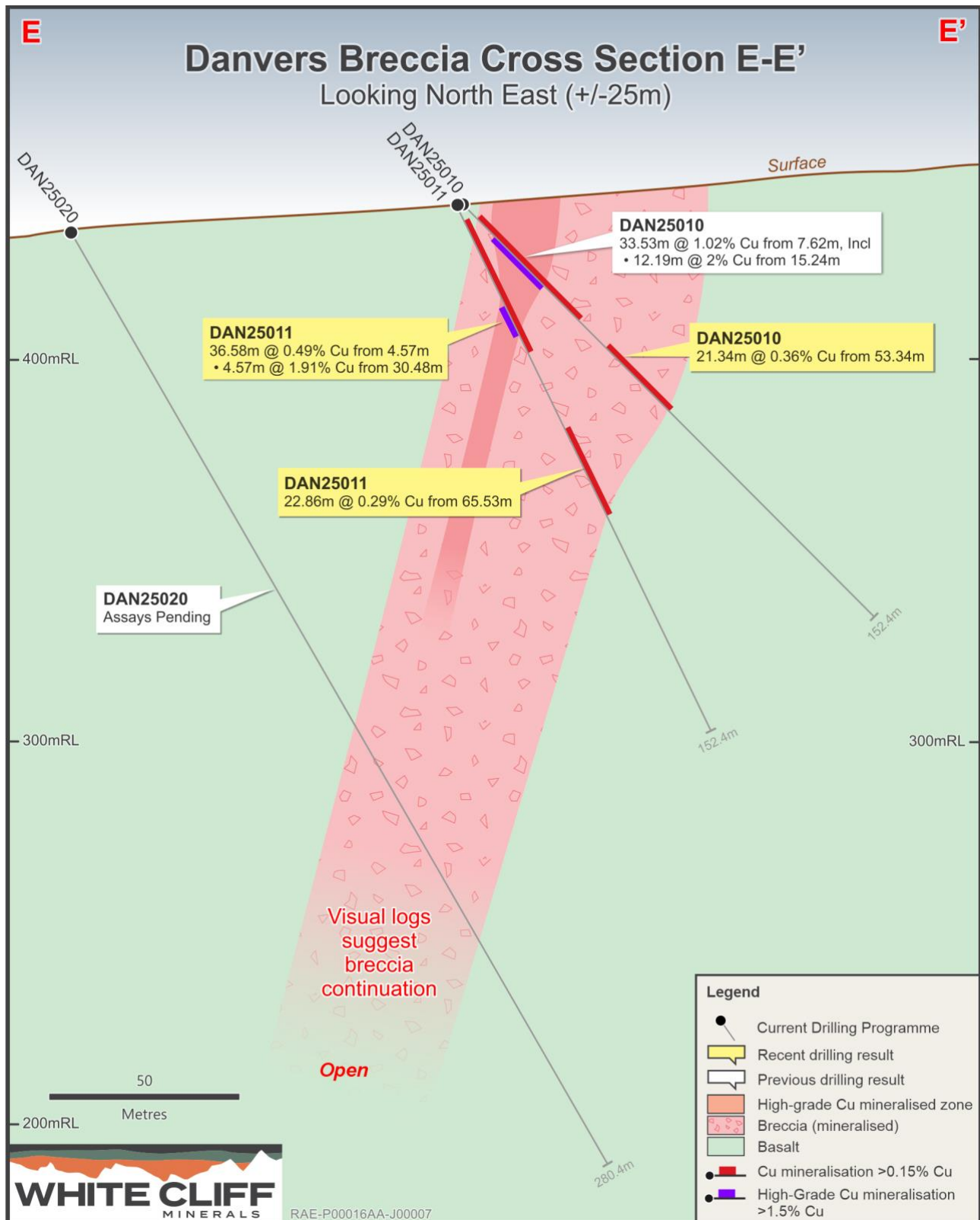
Figure 3 - Cross Section of drillholes DAN25010 and DAN25011 which intercepted a shallow zone of copper mineralisation. Assays are pending for drillhole DAN25020 which undercuts both drillholes, testing deep extensions to the known mineralisation.
