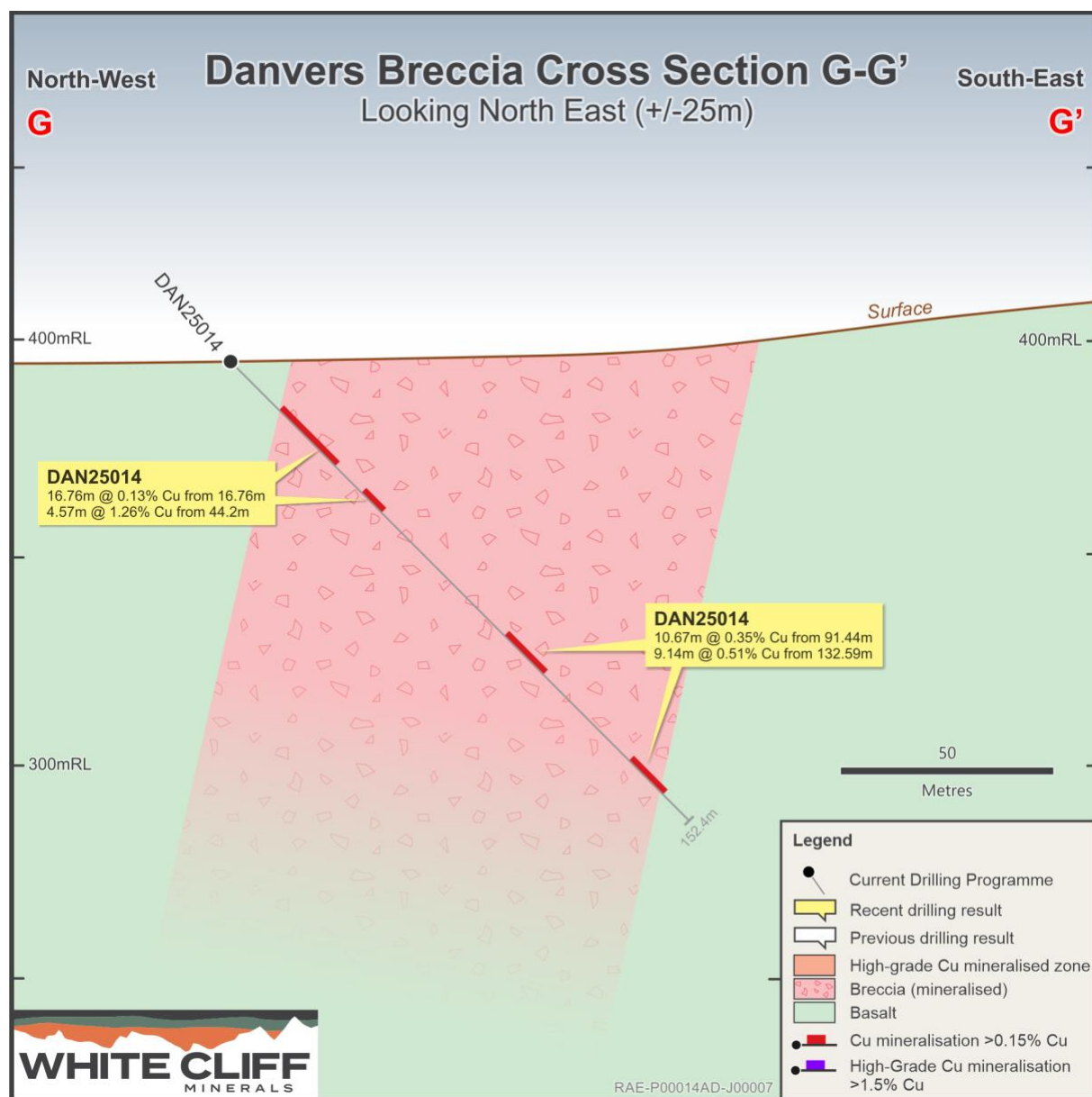
Figure 4 - Cross section of Drillhole DAN25014 which is 65m SW outside of the historic estimate footprint.
