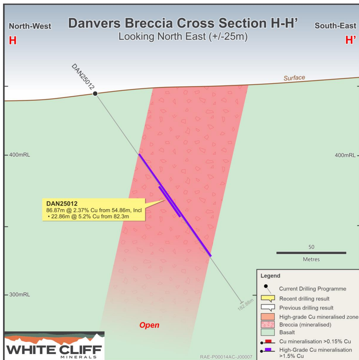
Figure 2 - Cross Section of drillhole DAN25012 which intercepted a shallow and thick high grade zone of copper mineralisation.
