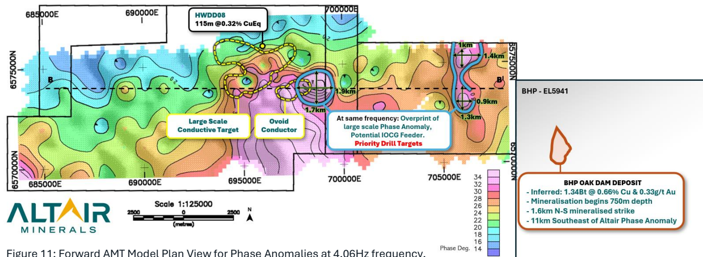
Figure 11: Forward AMT Model Plan View for Phase Anomalies at 4.06Hz frequency, with two major conductive targets. Model generated by Adelaide Mining Geophysics Pty Ltd. 2,3
