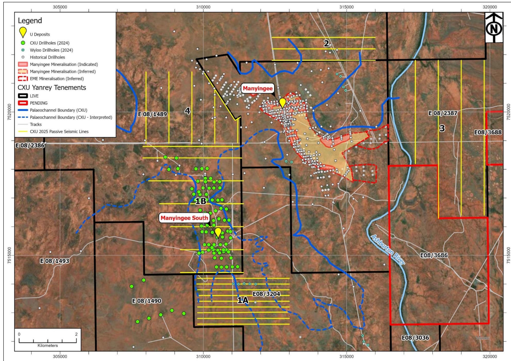
Figure 5. Cauldron Passive Seismic survey lines and areas.
