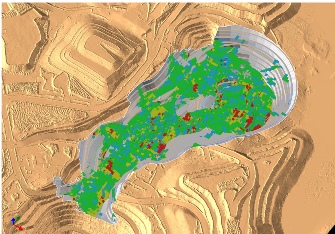
Figure 16. Jupiter Ore Reserve Layout
