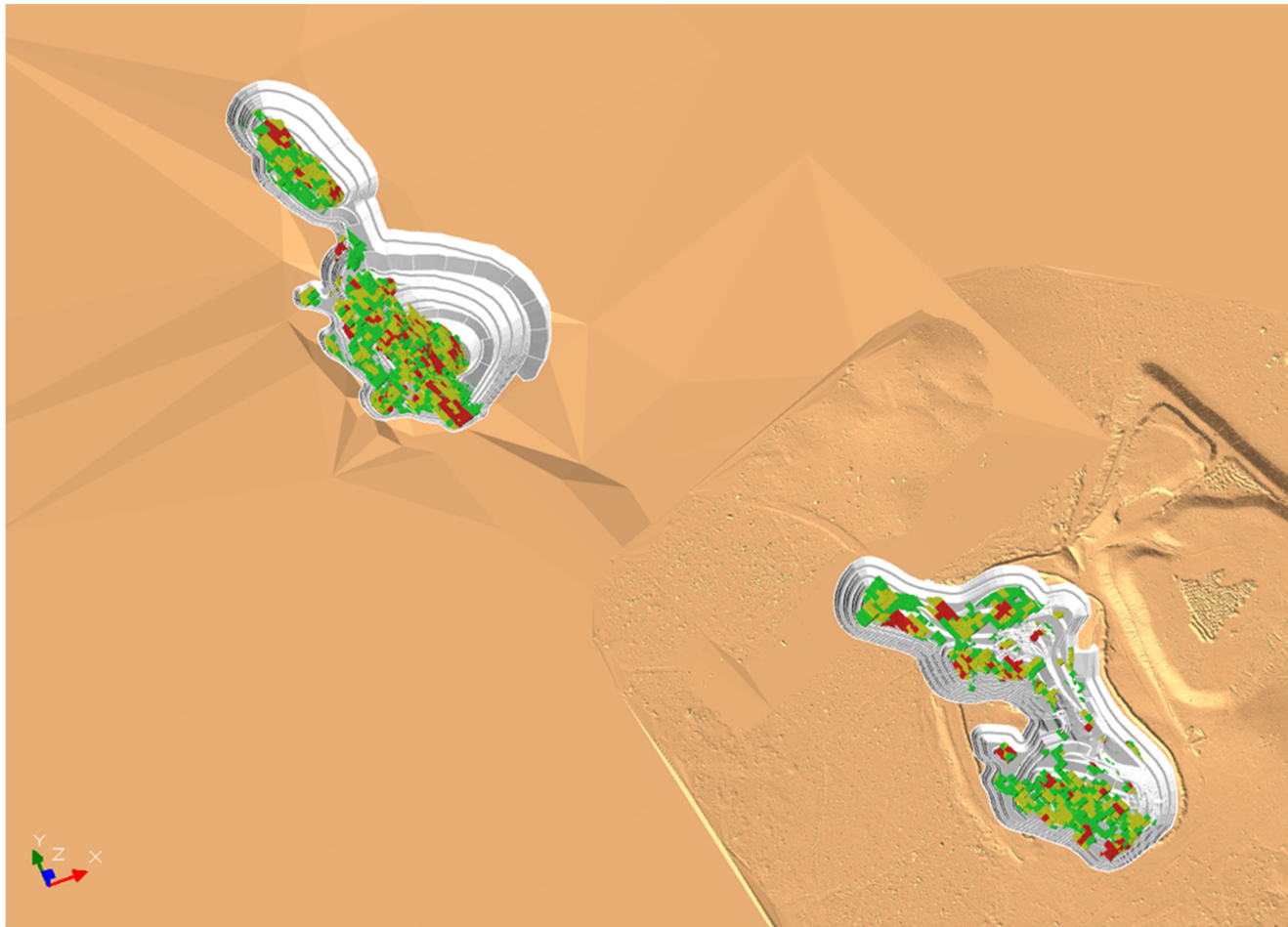
Figure 19. Puzzle and Puzzle North Reserve Pit Designs
