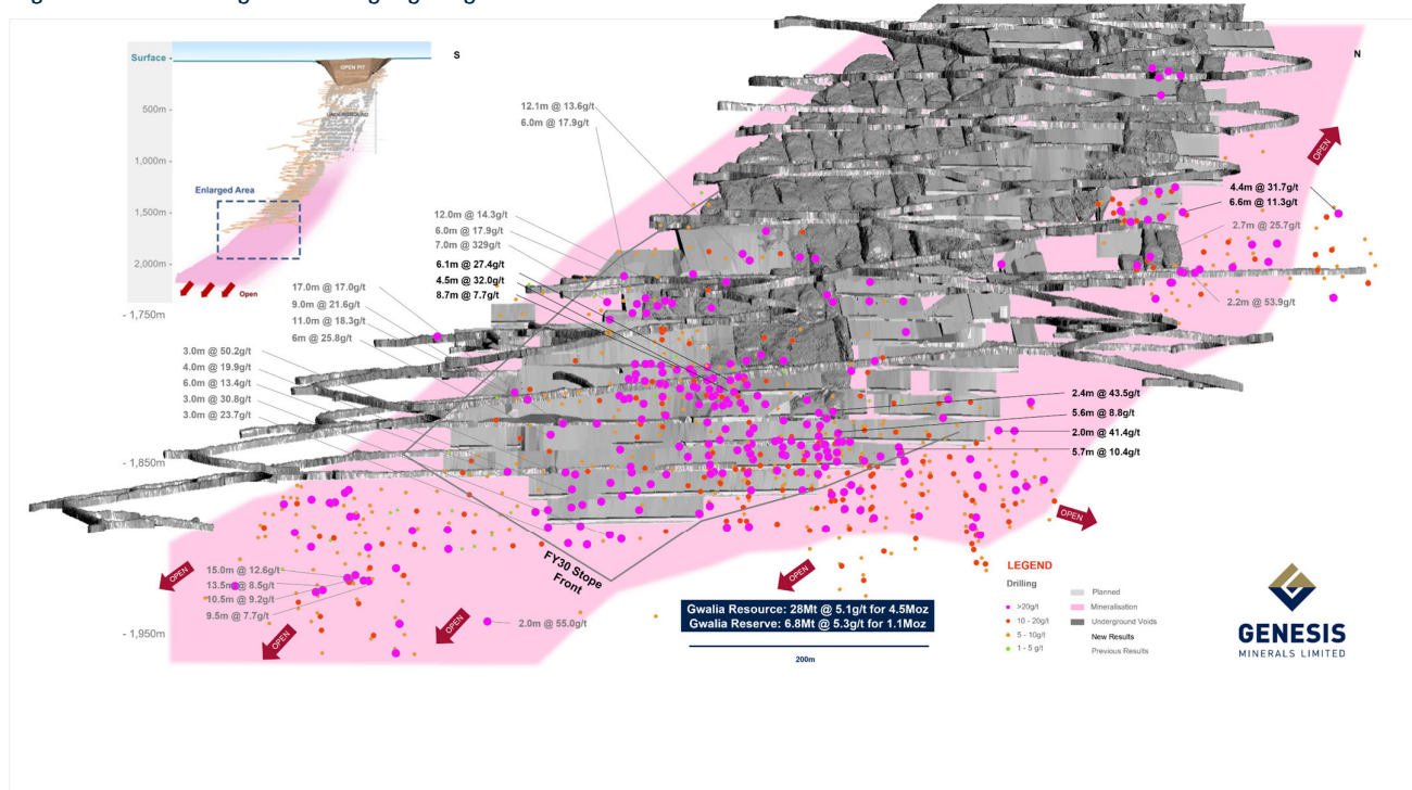
Figure 5. Gwalia long section highlighting drill results
