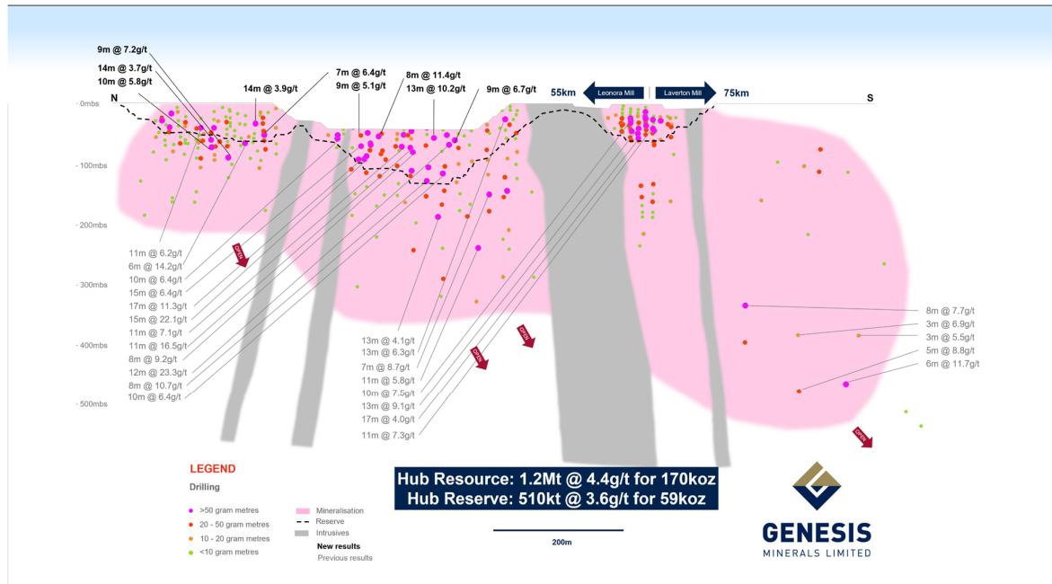
Figure 7. Hub long section highlighting drill results
