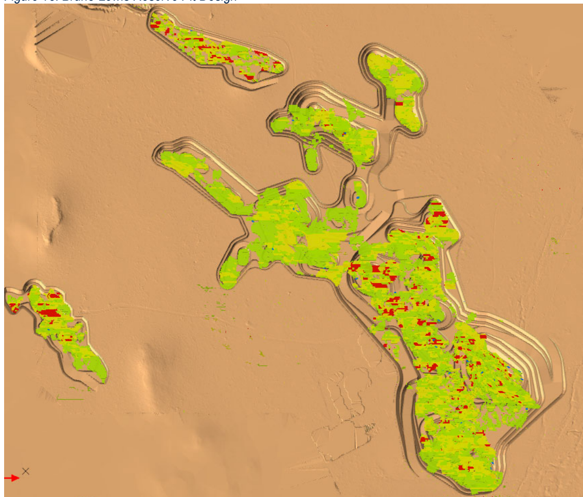
Figure 18. Bruno-Lewis Reserve Pit Design
