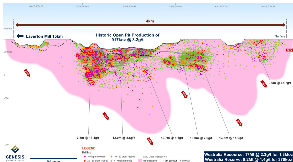
Figure 1. Westralia long section highlighting open pit Reserve
