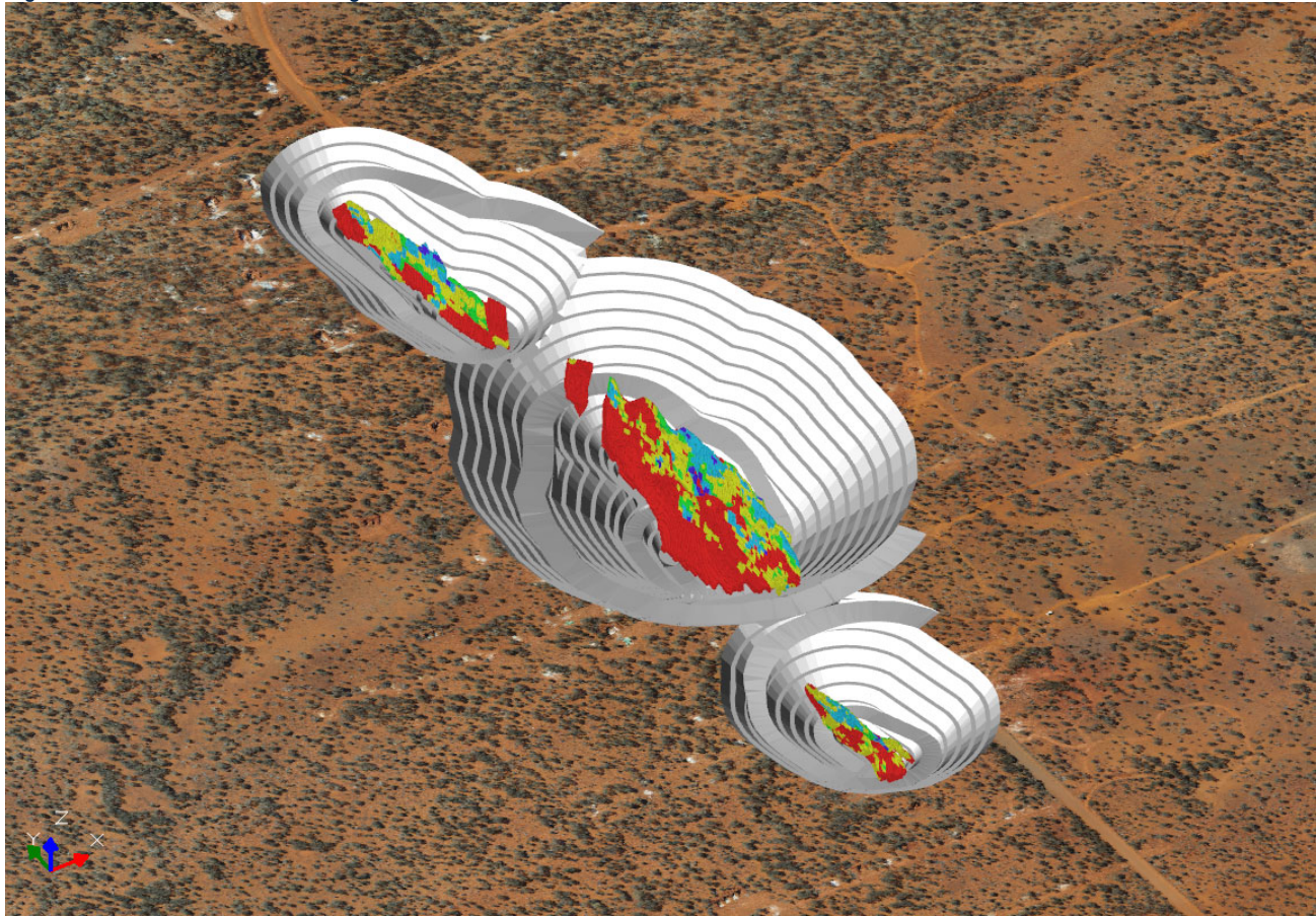
Figure 14. Hub Reserve Pit Designs
