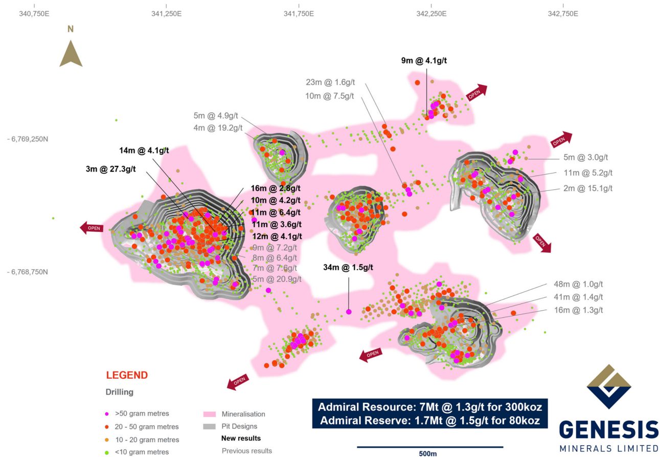
Figure 6. Admiral plan view highlighting drill results
