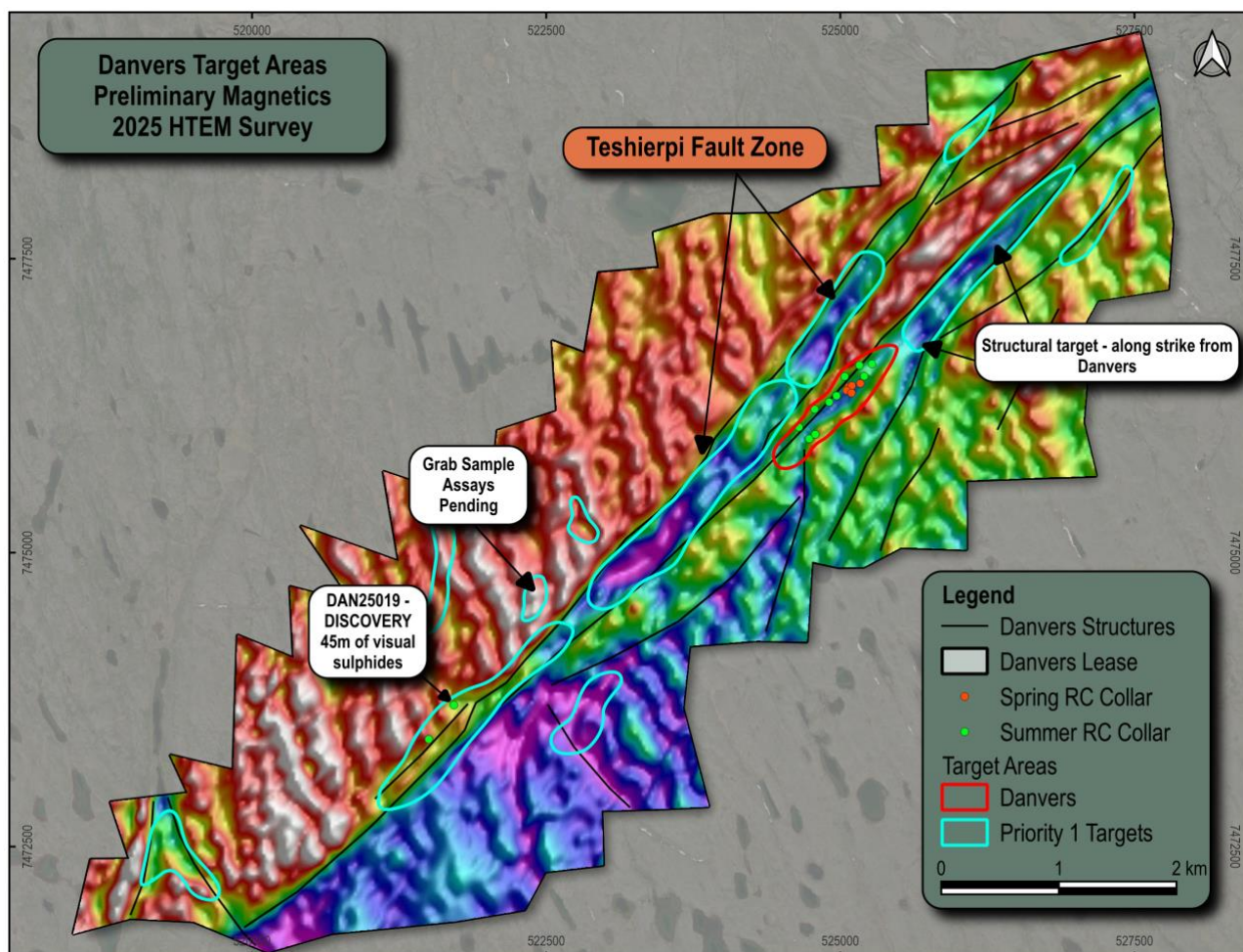
Figure 2 - Map of preliminary magnetic data for the Danvers Project, collect during the 2025 Heli-TEM survey. Newly identified targets are highlighted along strike of Danvers and in similar structural/magnetically quiet zones within the regional Teshierpi Fault Zone, which trends NE/SW over 10km through the Project. (Magnetic basemap is reduced to pole, total magnetic intensity with a NE sun shade overlying DEM. NAD83/UTM Zone 11N).
