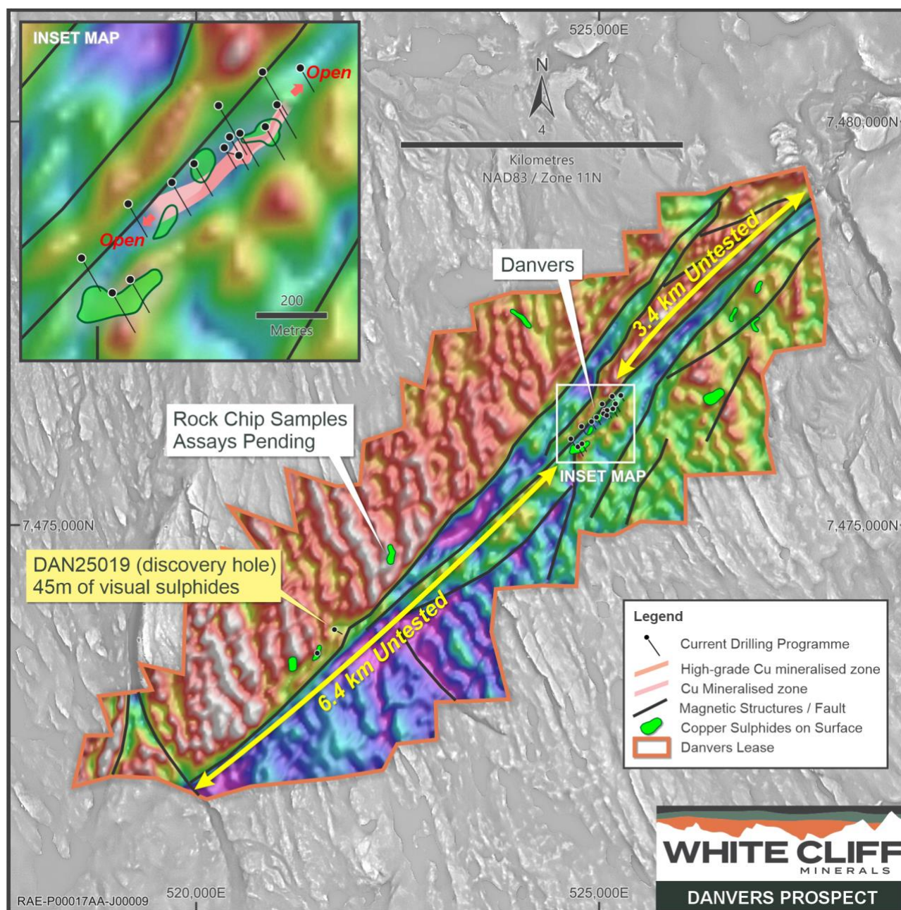
Figure 1 - Map of preliminary magnetic data for the Danvers Project collected during the 2025 Heli-TEM survey. Magnetic basemap is reduced to pole, total magnetic intensity with a NE sun shade overlying a DEM. (NAD83/UTM Zone 11N)
