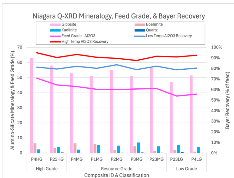
Figure 6. Niagara Bauxite Composites – Quantitative XRD Mineralogy for Alumino-Silicates, Feed grade ( \text{Al}_2\text{O}_3 %), and Bayer digestion recovery results expressed as % of feed grade
