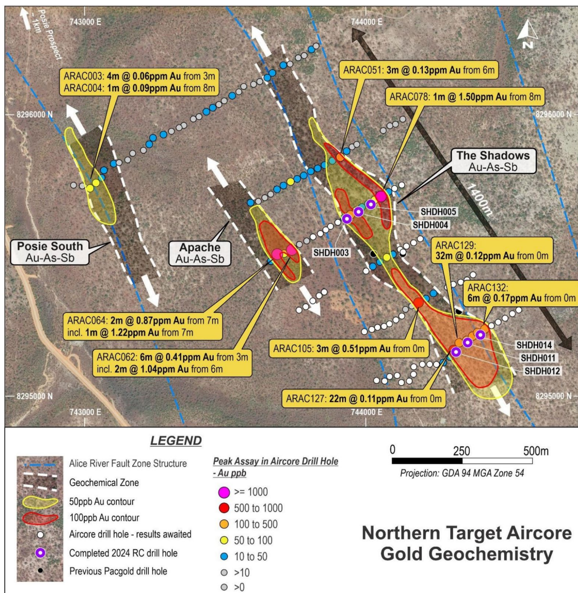
Figure 4: Au assays in Aircore programme at “The Shadows” delineates consistent mineralisation corridor over 1.4km in strike with new parallel zone previously unidentified. RC collars shown are recently completed with samples now in the laboratory
