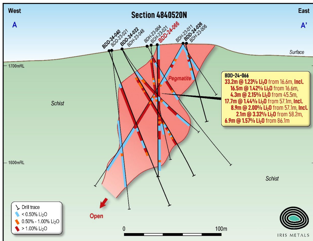
Figure 2: Section A-A'
