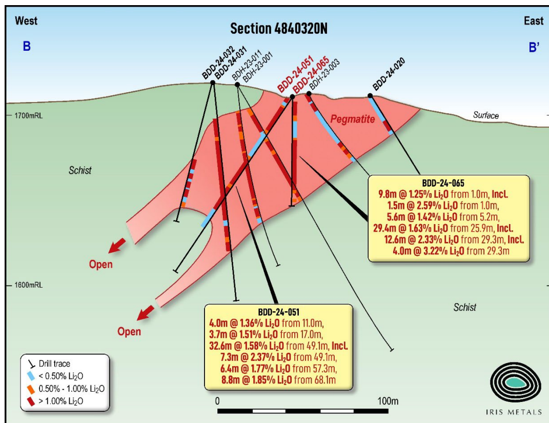
Figure 3: Section B-B'
