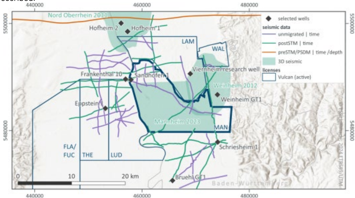
Figure 3: Mannheim licence 2D and 3D seismic coverage
