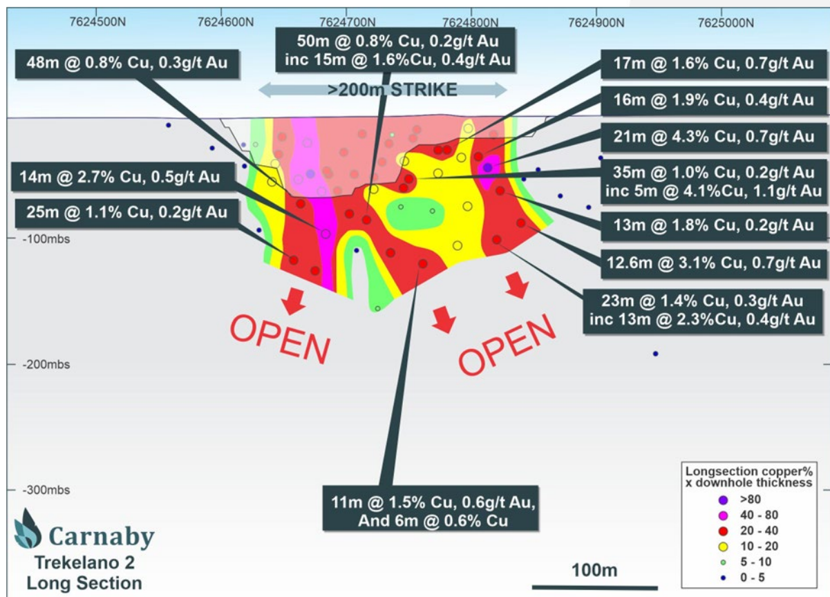
Figure 6. Trekelano 2 Long Section.
