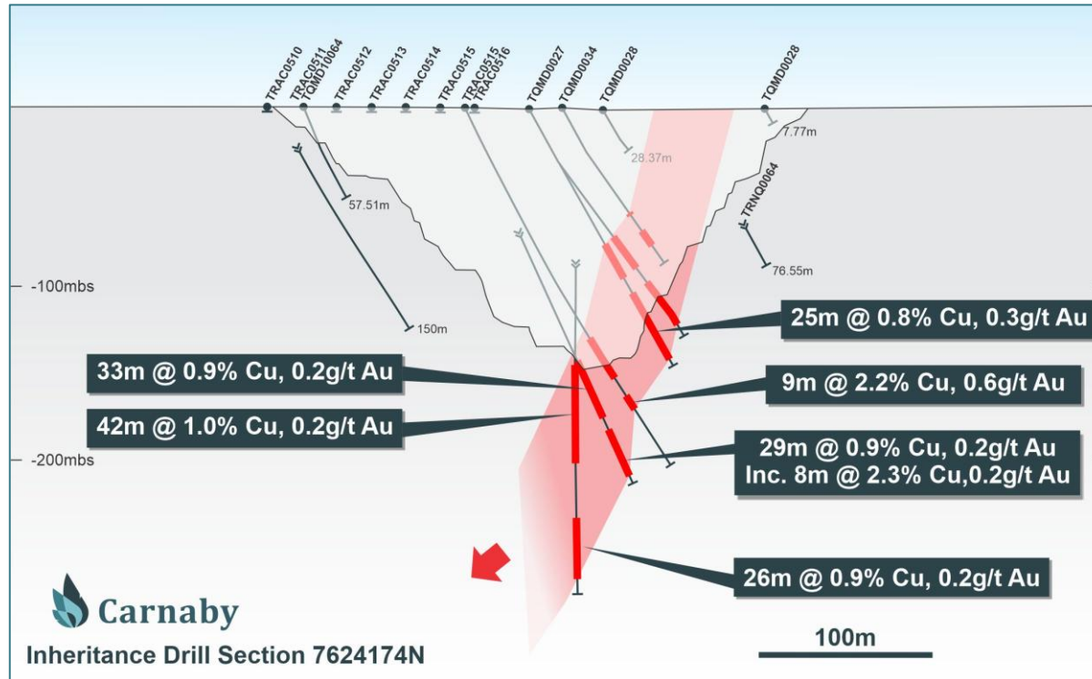
Inheritance Drill Section 7624174N
