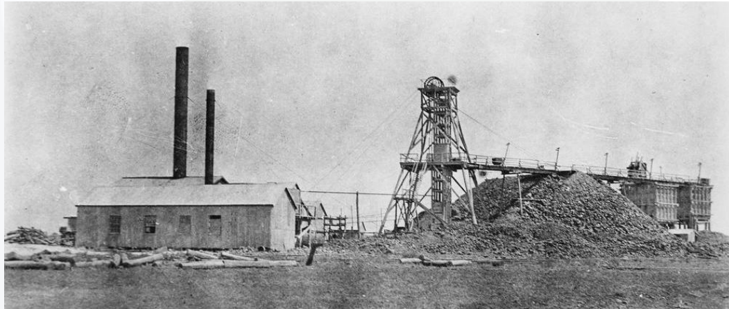
Trekelano – Cloncurry mining fields longest continuous producer (from 1911-1945) - produced 188,000t @ 10.9% Cu
