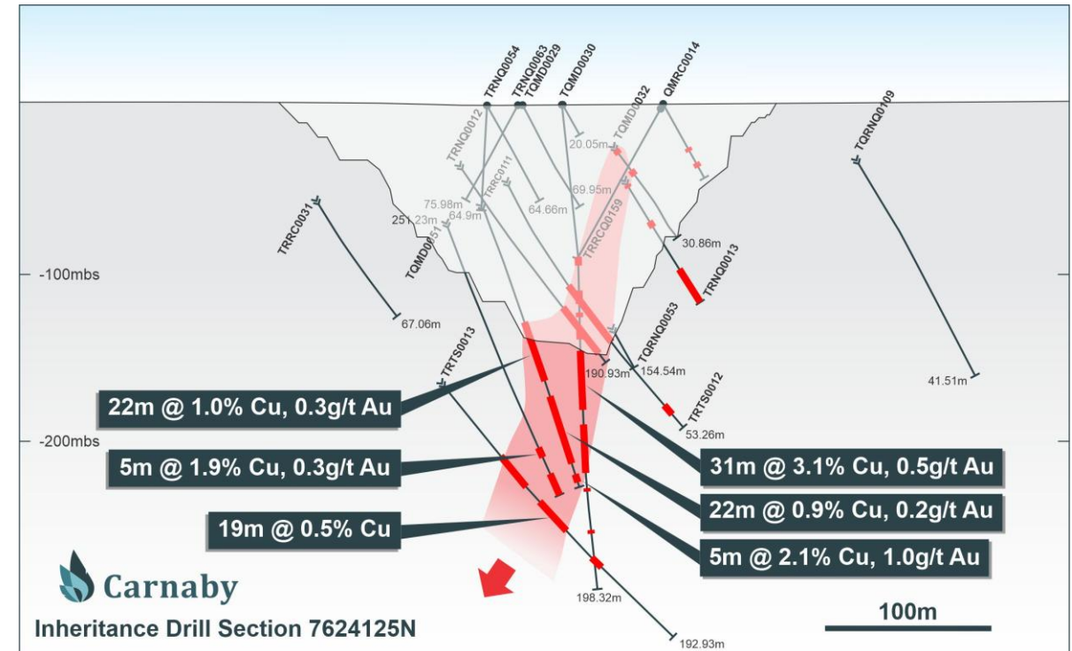
Inheritance Drill Section 7624125N
