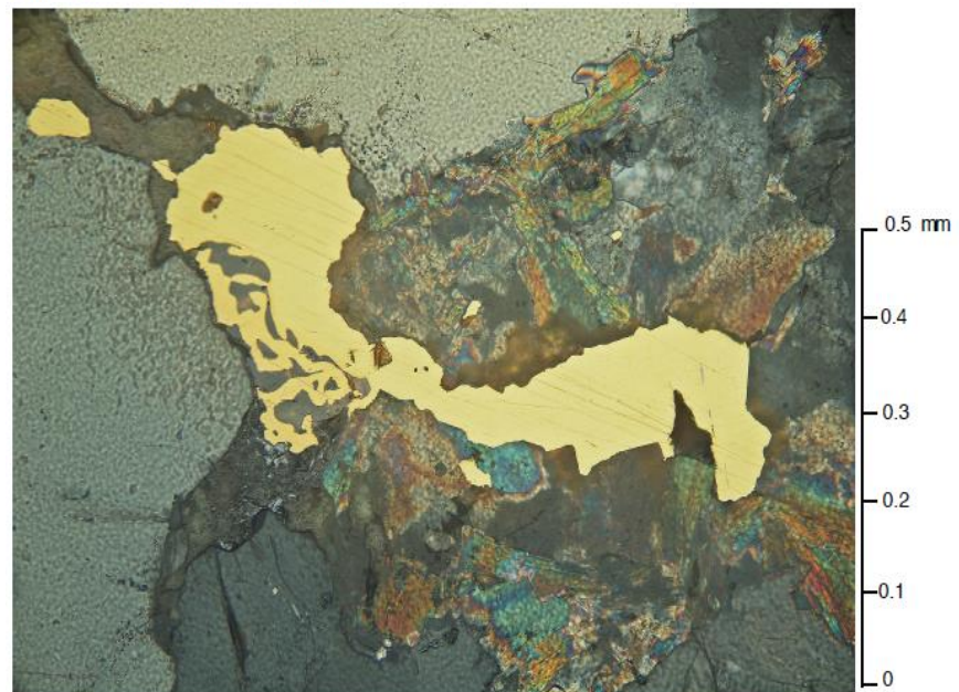
FIG. 9: SAMPLE SOM-HS2 (Combined transmitted and reflected light, crossed polarisers, Obj. x20, Image P6068589). This view illustrates a large ragged grain of native gold (bright yellow), with smaller grains, embedded in a dense sericite alteration aggregate (brightly coloured flakes).
