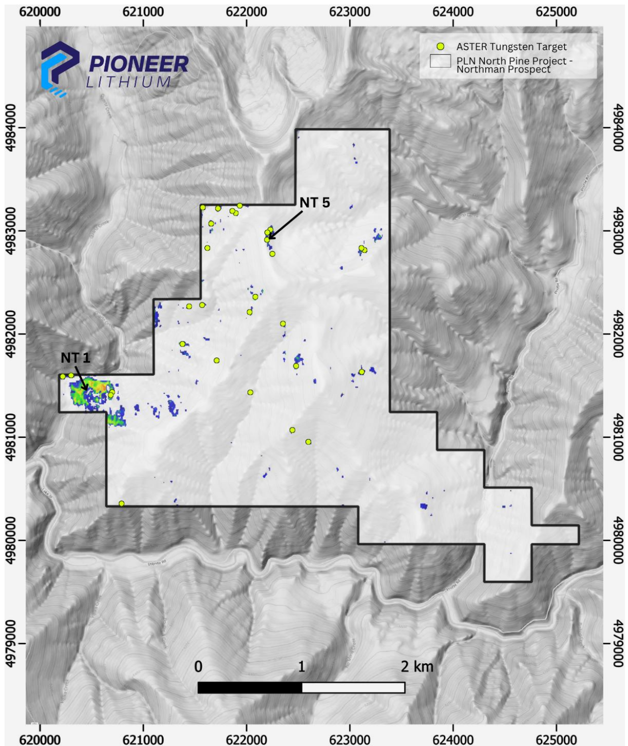
Figure 7: ASTER spectral analysis showing tungsten only signatures currently being investigated by Pioneer's field geologists. Target NT 1 is co-incidental with antimony signatures while NT5 represents a tungsten only target.
