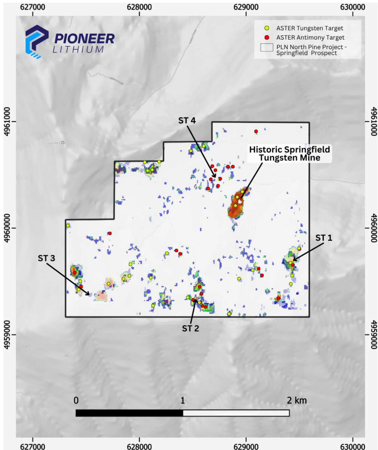
Figure 2: ASTER analysis showing the location of antimony and tungsten indicators at Springfield Prospect. Multiple co-incidental signatures occur in the south of the claim group located uphill from the existing known mineralisation ST1 – ST3).
