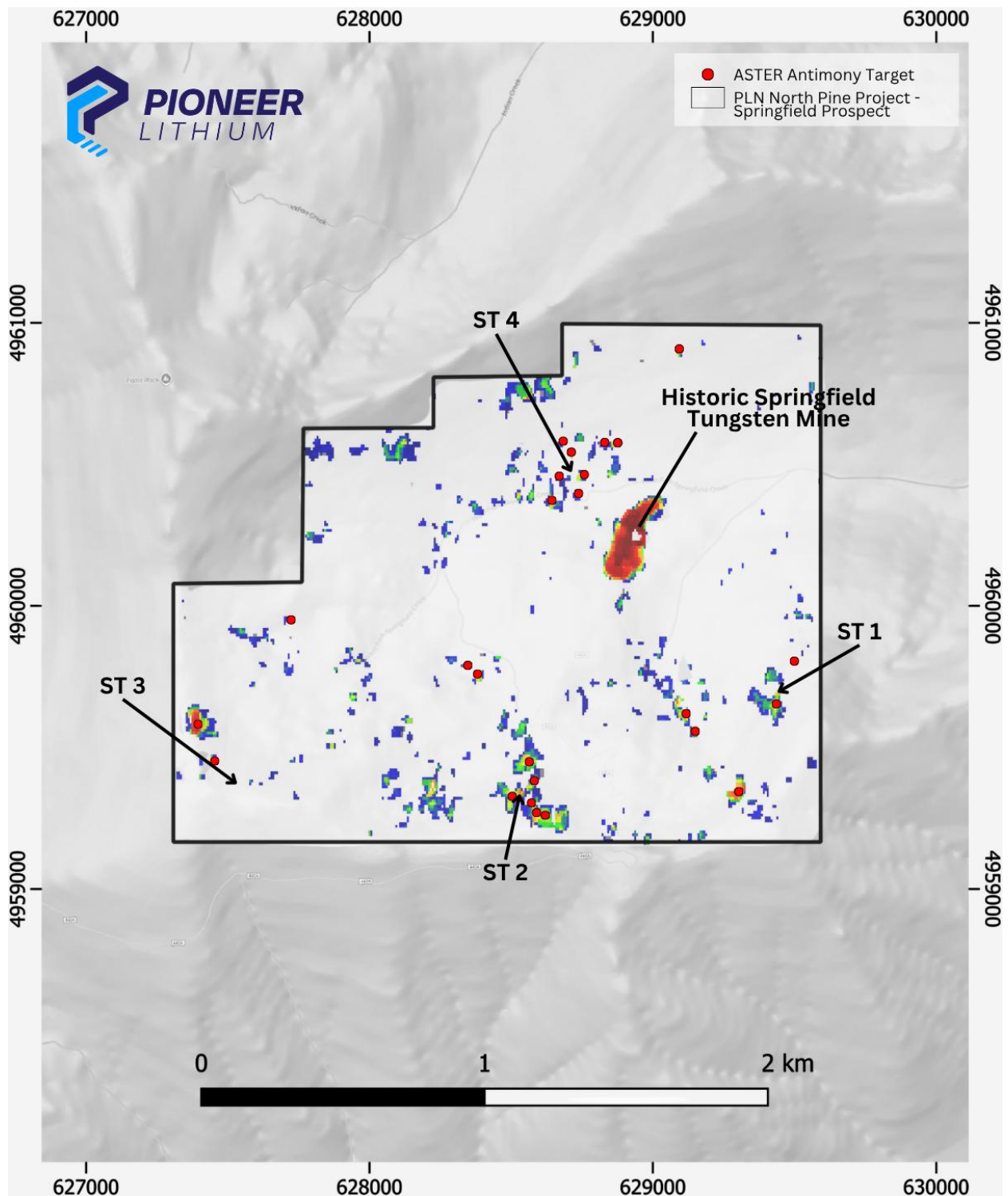
Figure 3: ASTER spectral analysis showing antimony targets currently being investigated by Pioneer's field geologists, note the cluster of targets occurring NW and upstream of the Springfield Mine at ST4.
