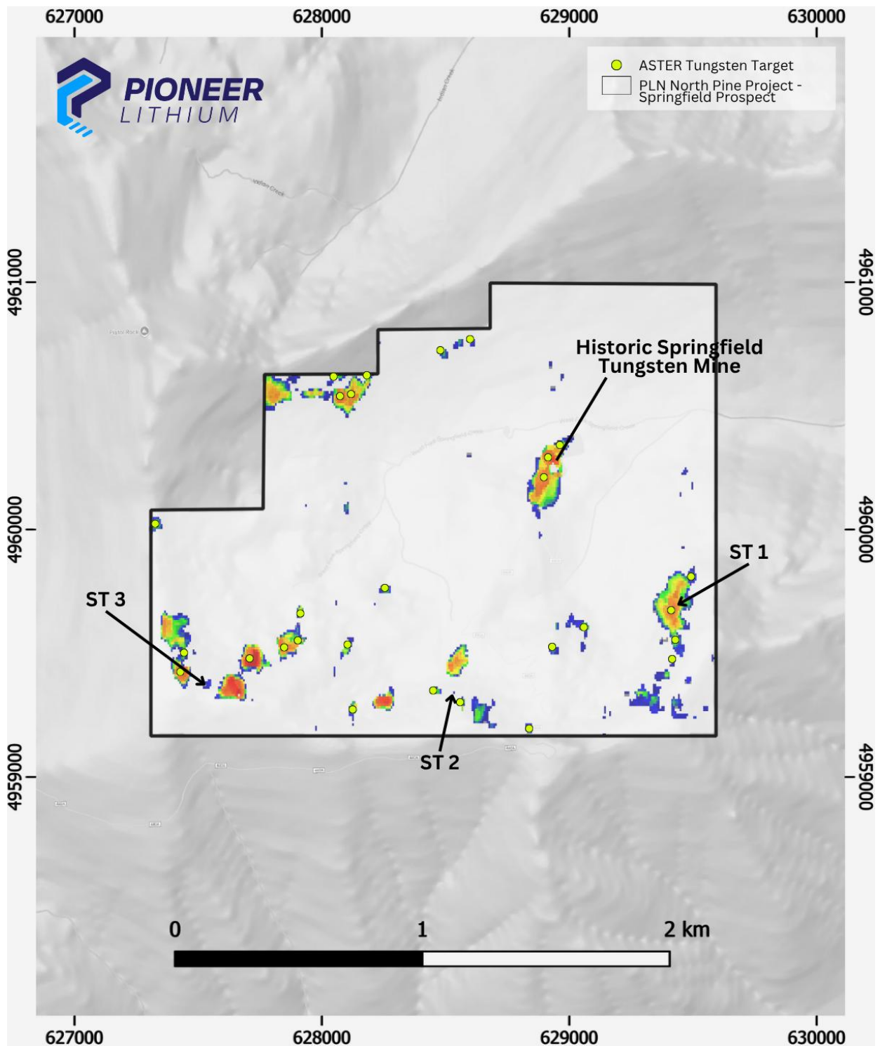
Figure 4: ASTER spectral analysis for mineral endmembers indicative of tungsten mineralisation, note the strong ASTER targets to the south of Springfield Tungsten Mine with very similar strength of signal as the Springfield Tungsten Mine itself (ST1 and ST3).
