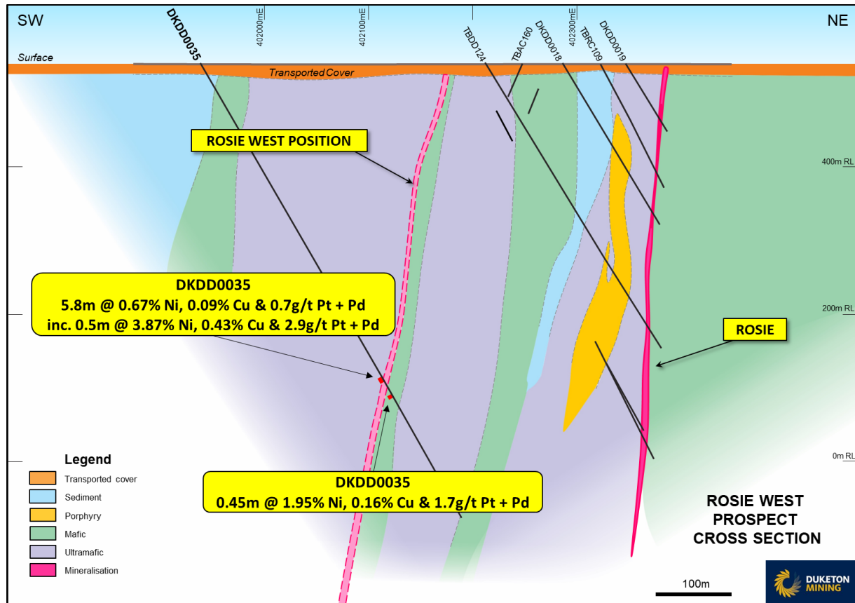
Figure 4: Cross section of DKDD0035, Rosie West
