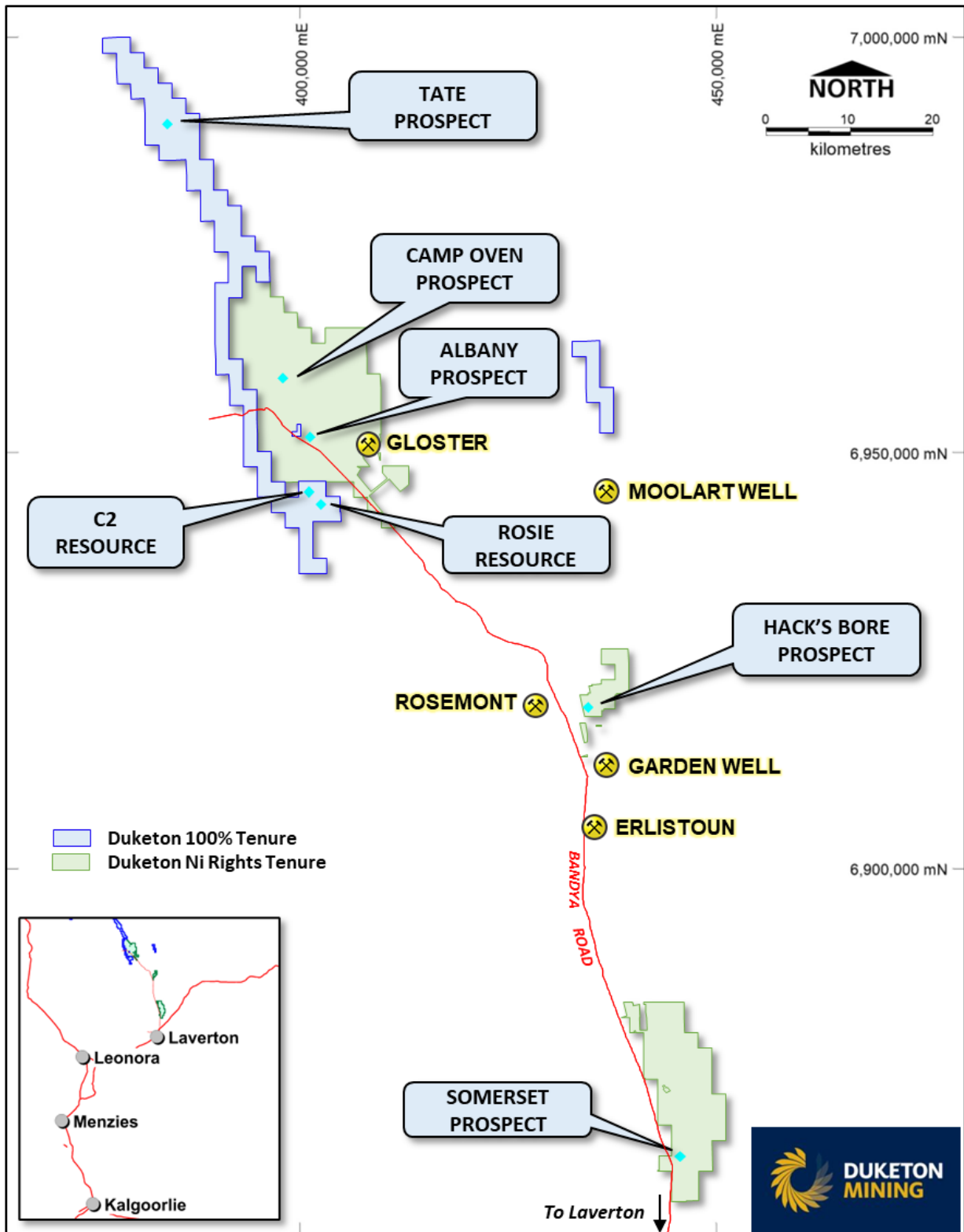
Figure 5: Location map of the Duketon tenement holdings and location of the DKM prospects
