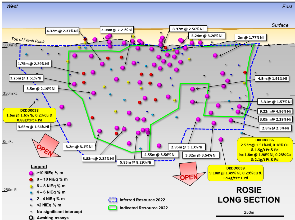
Figure 3: Rosie Long Section
