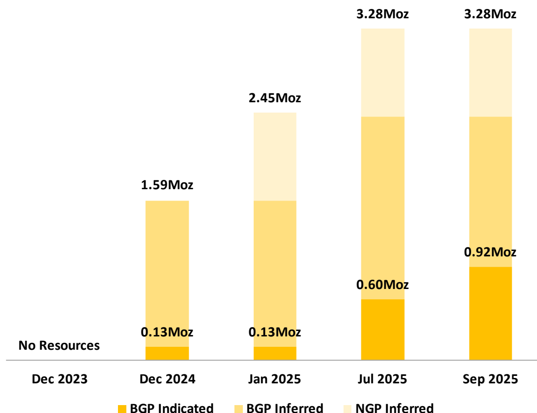
Figure 1: Group Mineral Resource timeline, global and Indicated ounces annotated (BGP = Boundiali Gold Project, NGP = Napié Gold Project)
