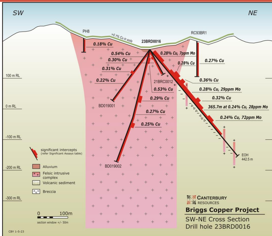
Figure 5 Cross Section for 23BRD0016, Briggs Central
