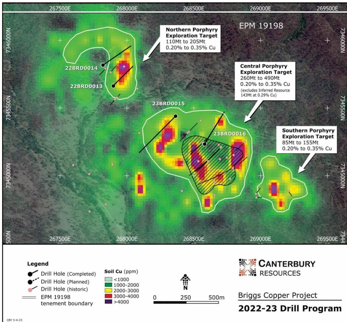
Figure 2 Plan displaying Exploration Target outlines based on 0.1% Cu-in-soil contour (white) and existing Inferred Mineral Resource outline (black), plus historic and recently completed drill holes
