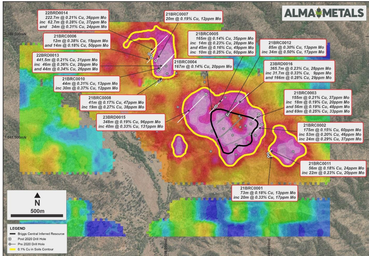
Figure 6 Plan showing 2021-2023 drilling, most of which lies outside the current Mineral Resource at Briggs Central
