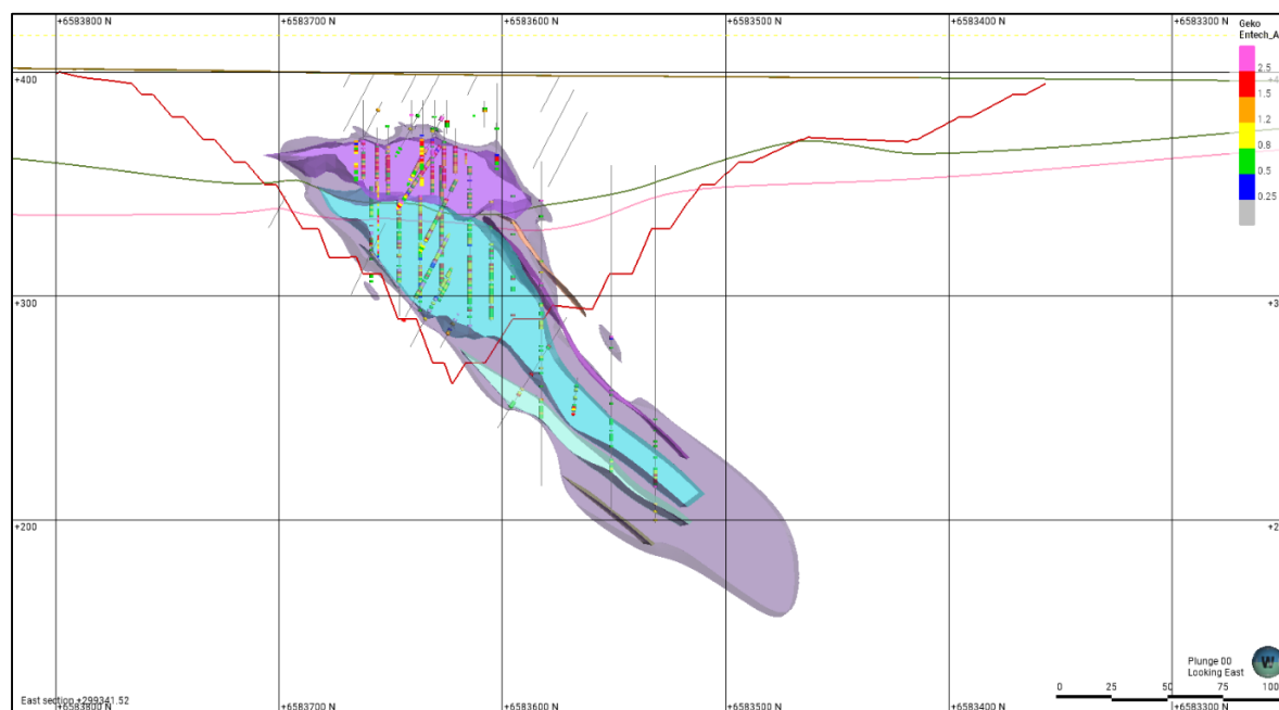
Figure 6: Typical cross section of Geko deposit (azimuth 90°) showing drill hole traces, mineralisation domains, weathering, topography, pit design and open pit interpretation extents
