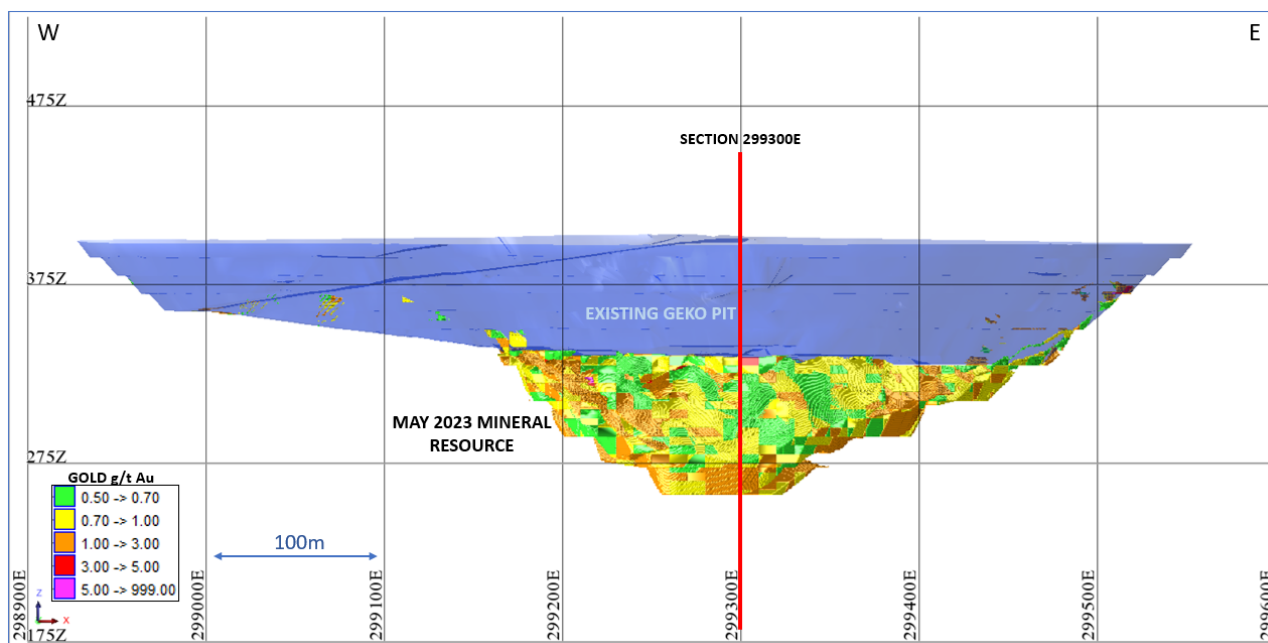
Figure 4: Long section view of Geko Open Pit with Mineral Resource model
