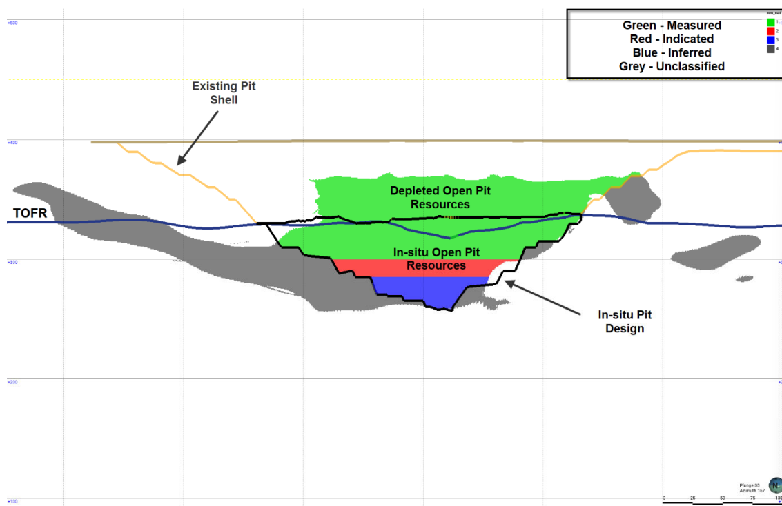
Figure 8: Long section (azimuth 167°) of the Geko deposit displaying extents of classified resources within the open pit
