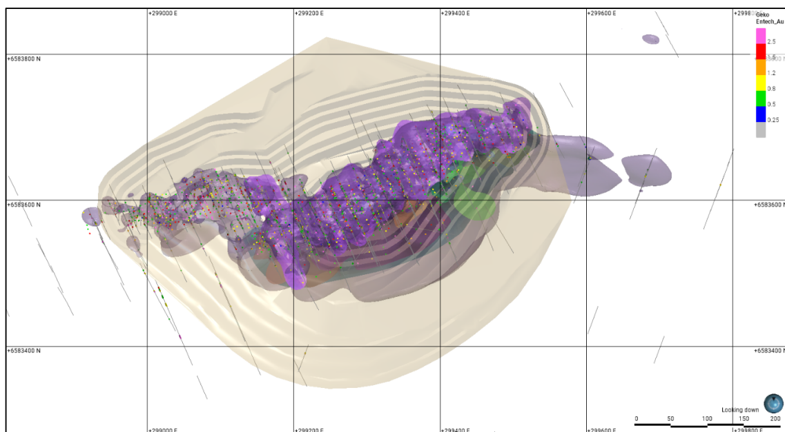
Figure 7: Plan section of Geko deposit showing drill hole traces, mineralisation domains and open pit void
