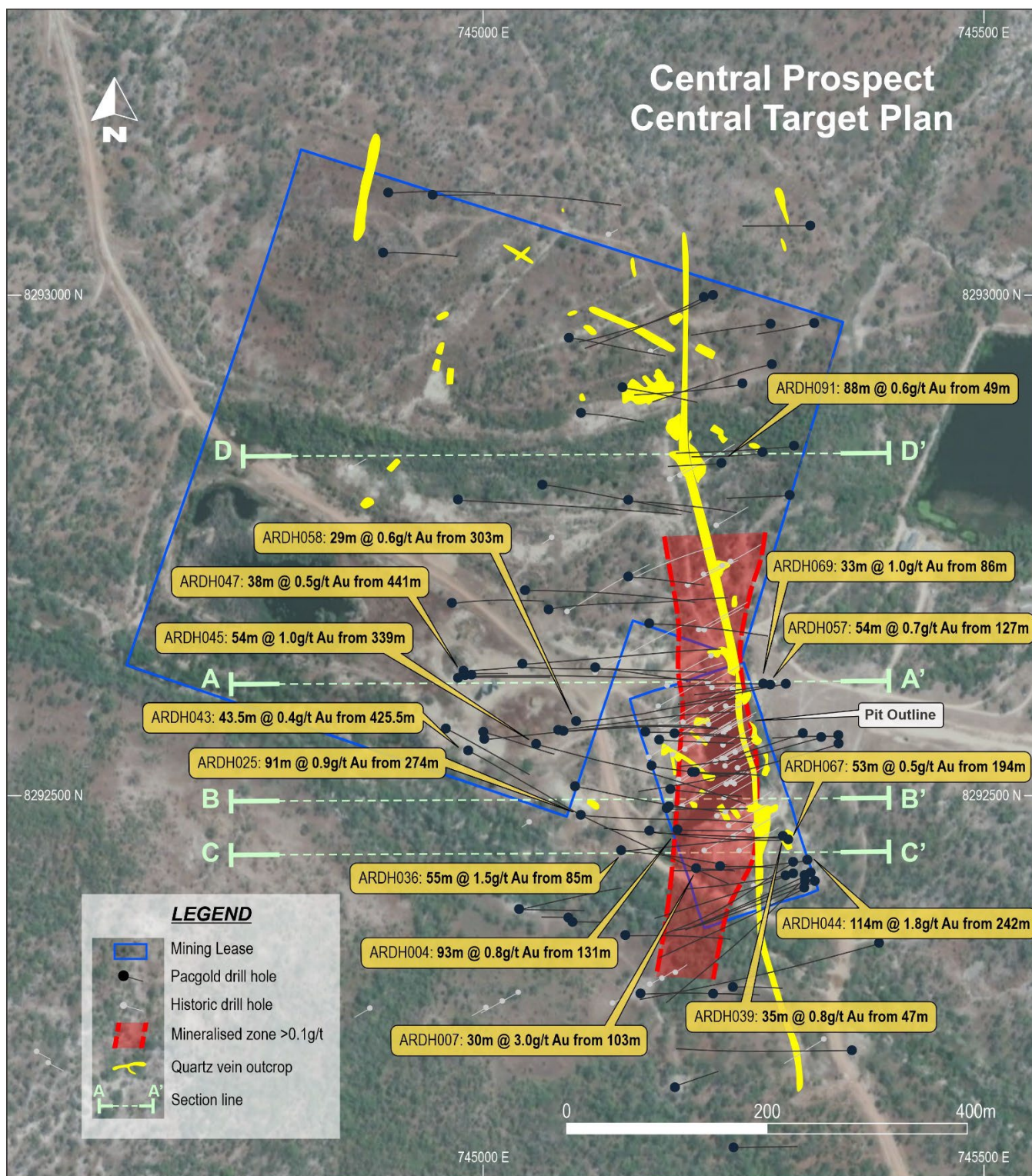
Figure 4; Plan view of drillhole traces at the Central Target zone with drillhole intersections and trace of mineralised body projected to surface overlain on satellite image
