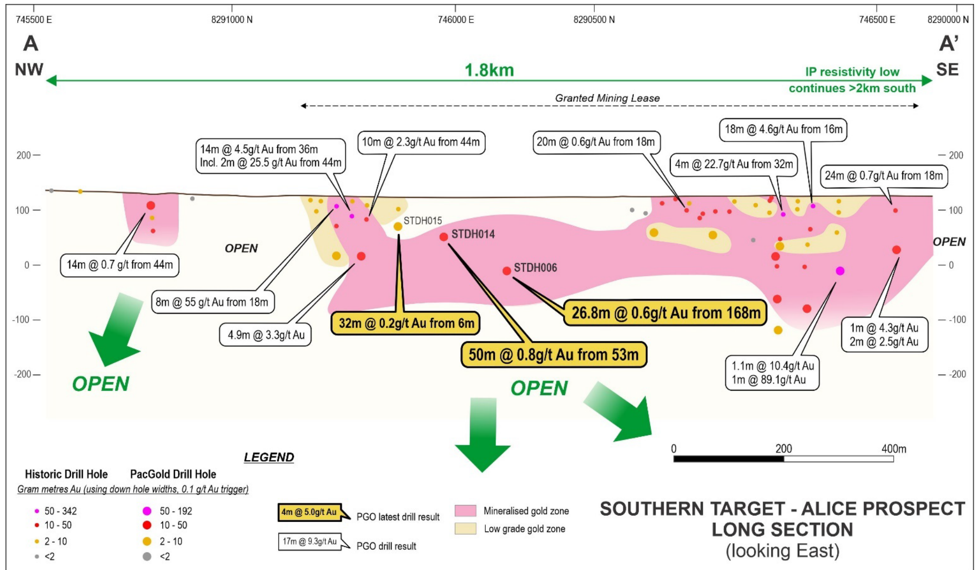
Figure 9; Long Section of Southern targets area with pierce points and gold contours (gm)
