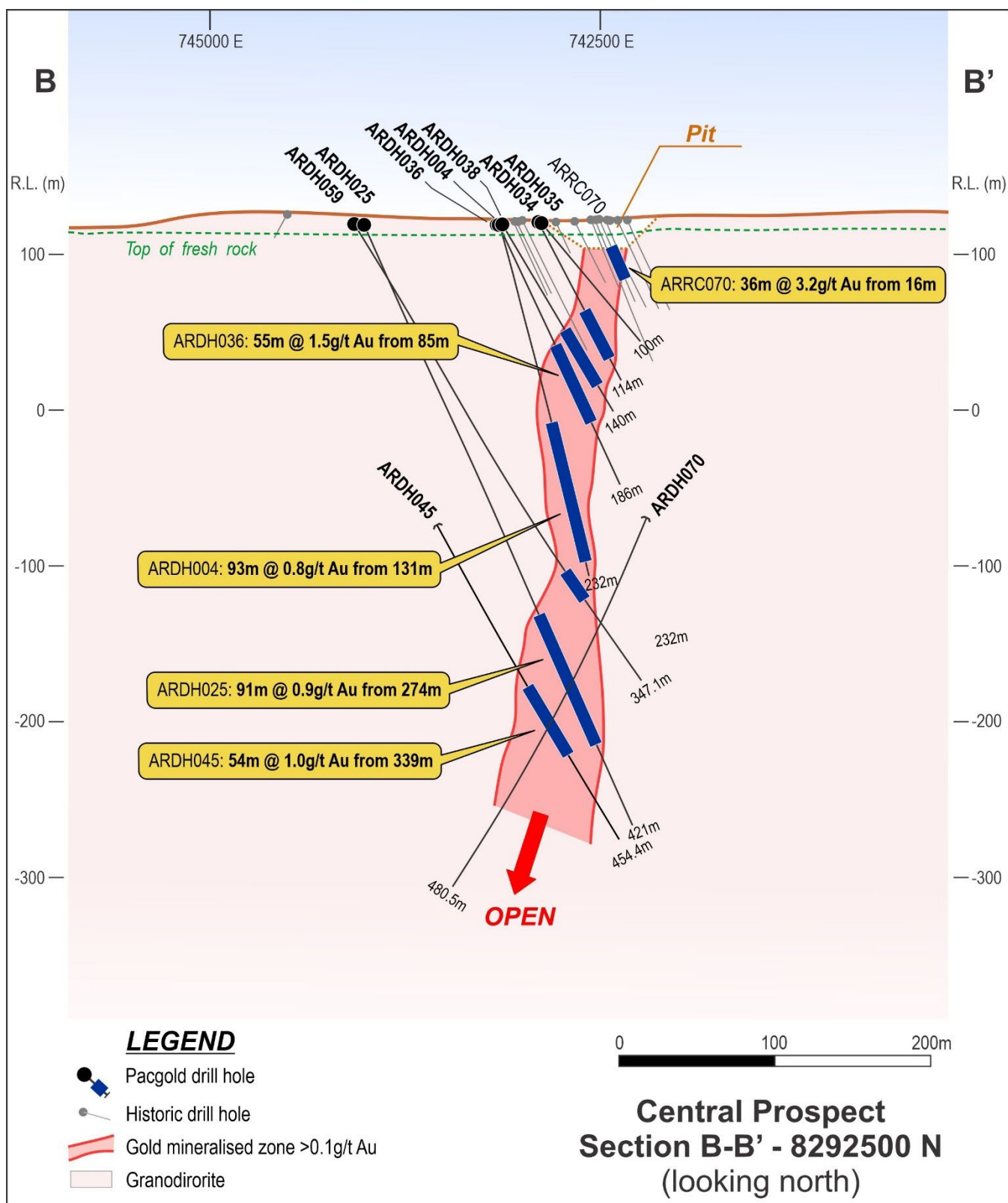
Figure 3; Cross Section B-B'-8292500N showing drillhole intersections and interpreted mineralised outline
