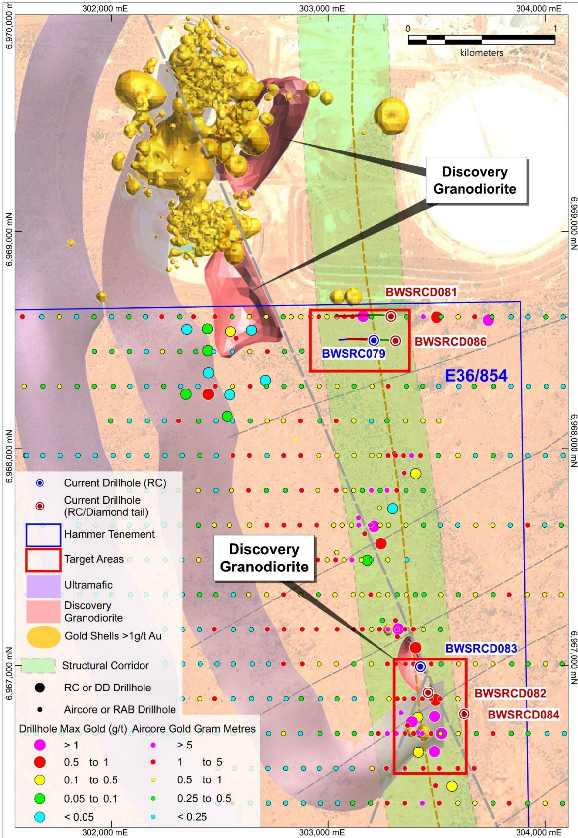
Figure 4. Plan view showing Eastern and Central Targets and their proximity to the Bronzewing anticlinal axis (Yellow dash) and the Eastern Sheer Zone (Grey Dashes). Historical air core coverage and anomalies also shown on the tenement (refer to ASX announcement 2 October 2019, 5 and 15 September 2025).
