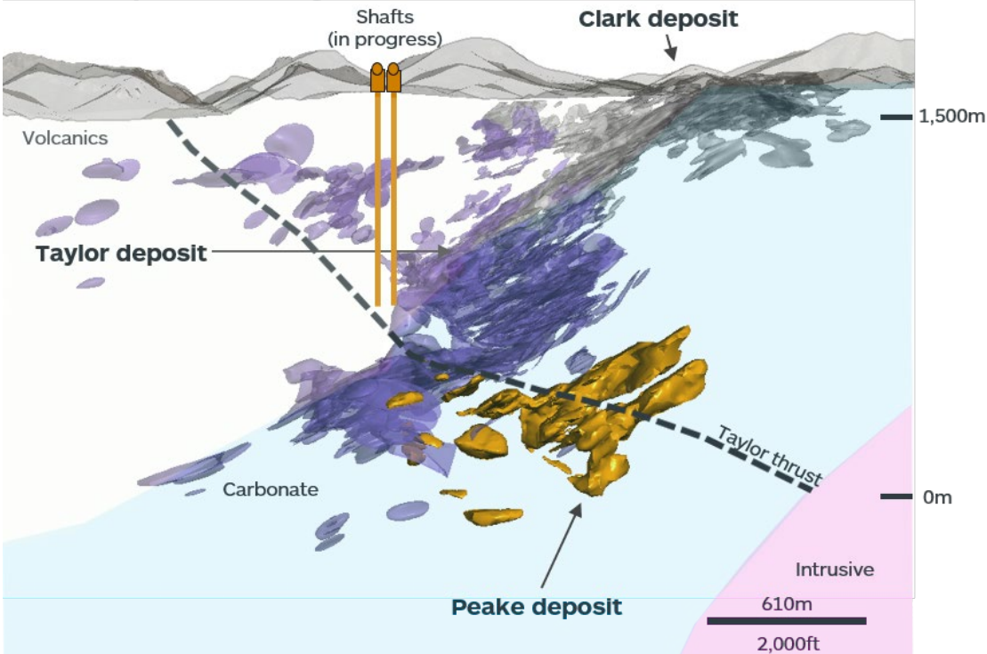
Peake deposit (looking east)
