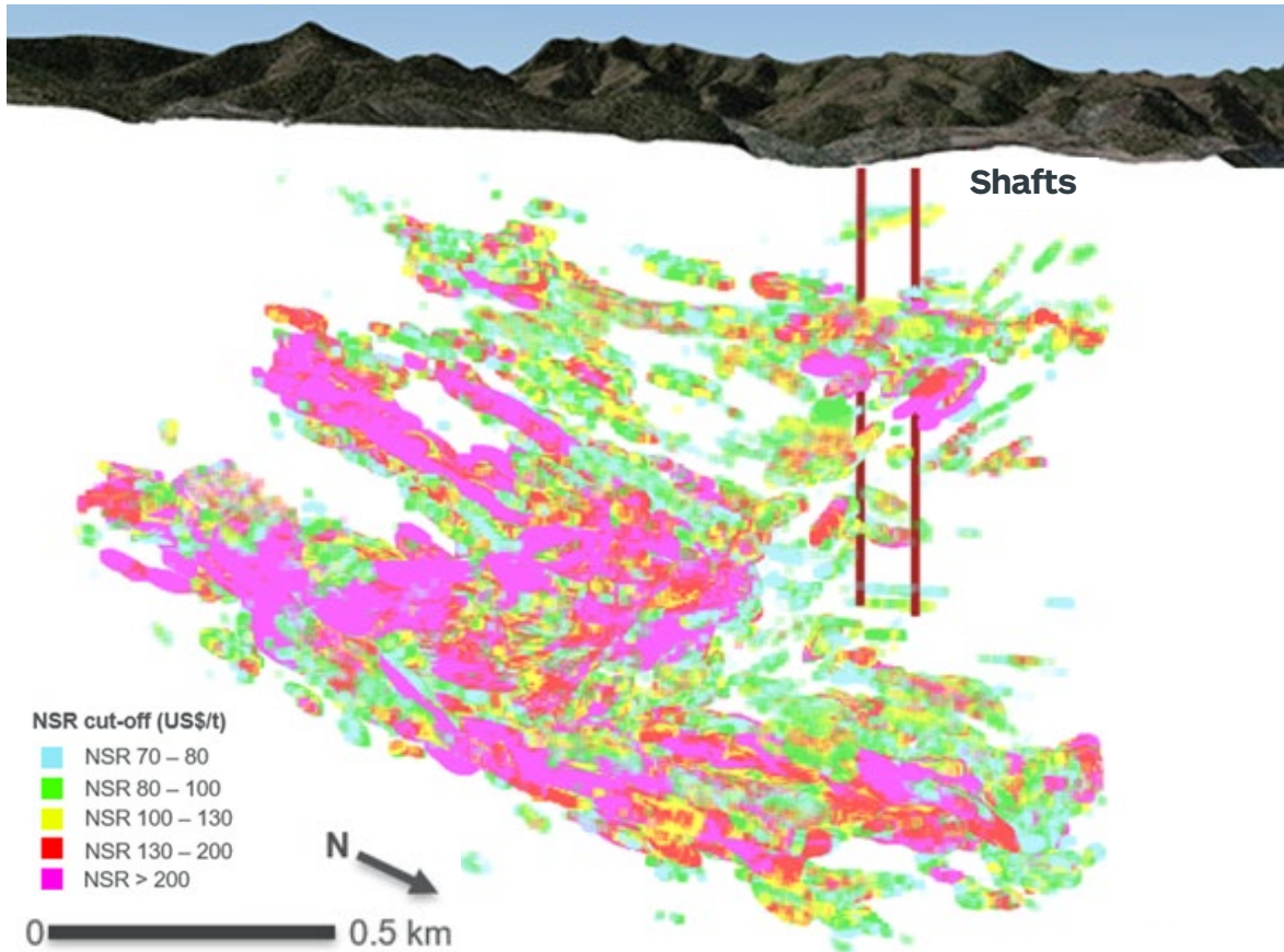
Taylor geology and mineralisation (looking southwest)
