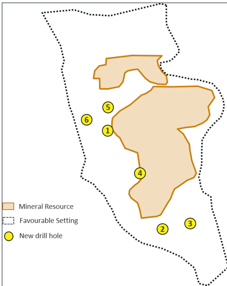
Figure 4: Plan view of the Peake Mineral Resource and favourable setting with newly reported exploration drill holes shown as circles where the holes intersected.
