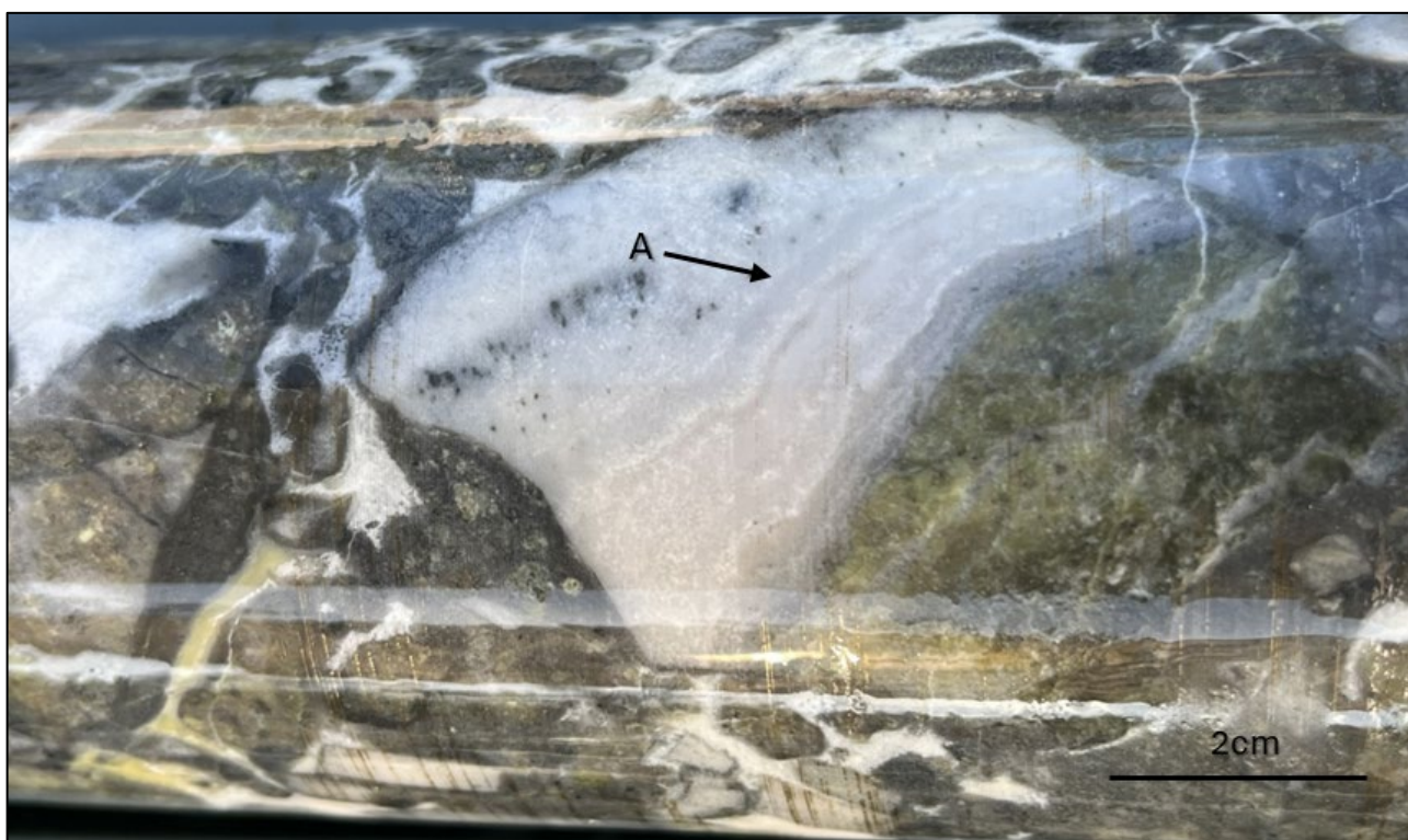
Figure 6: Hydrothermal breccia with rounded clast of epithermal crustiform - colloform banded veining (A) and black sulphide clasts within a broader matrix of calcite from Main Vein in 25FCDD014.
