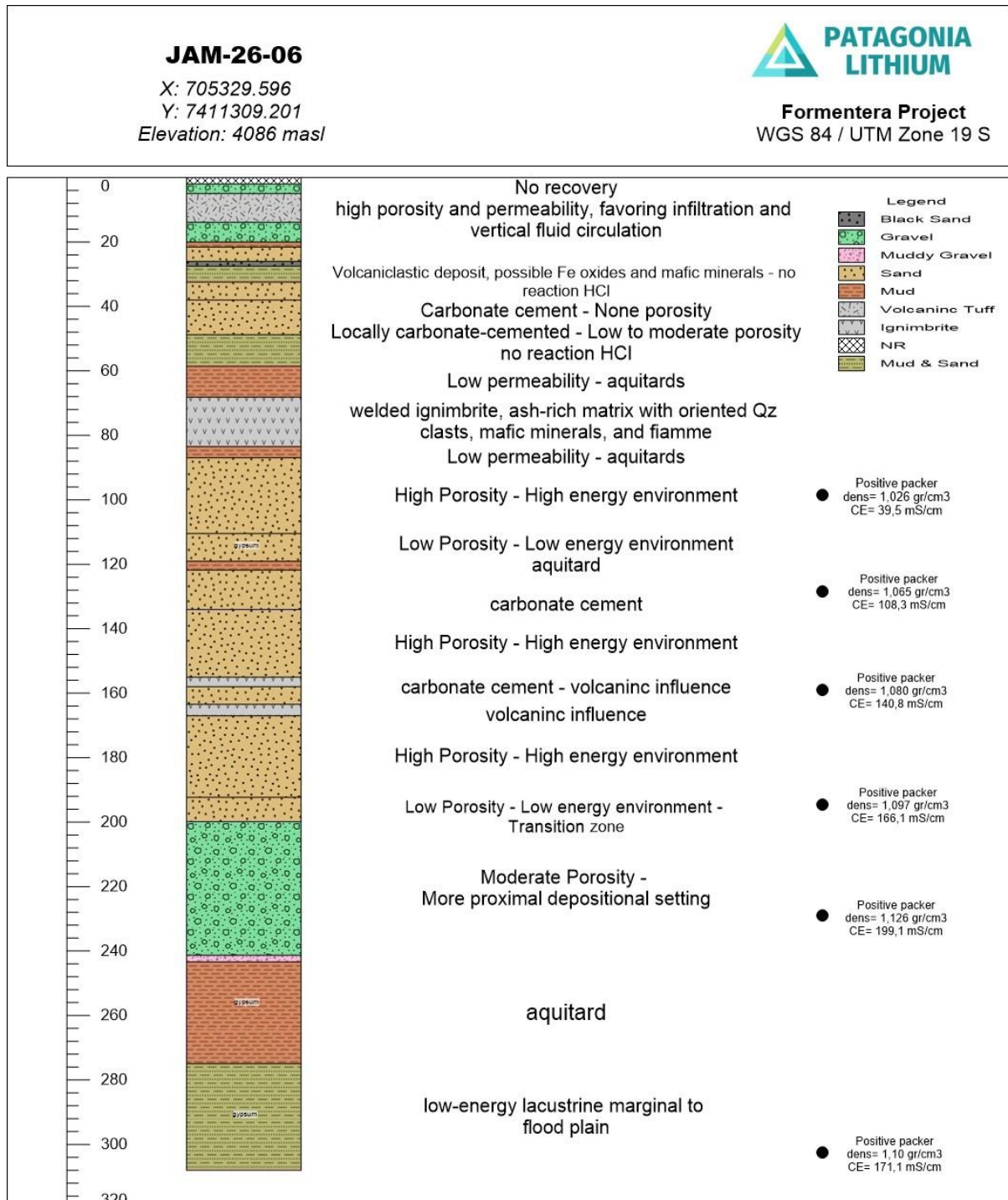
Figure 3. Lithology log of packer tests and visual descriptions. Porosity will be tested in the laboratory and later using BMR Gamma.
