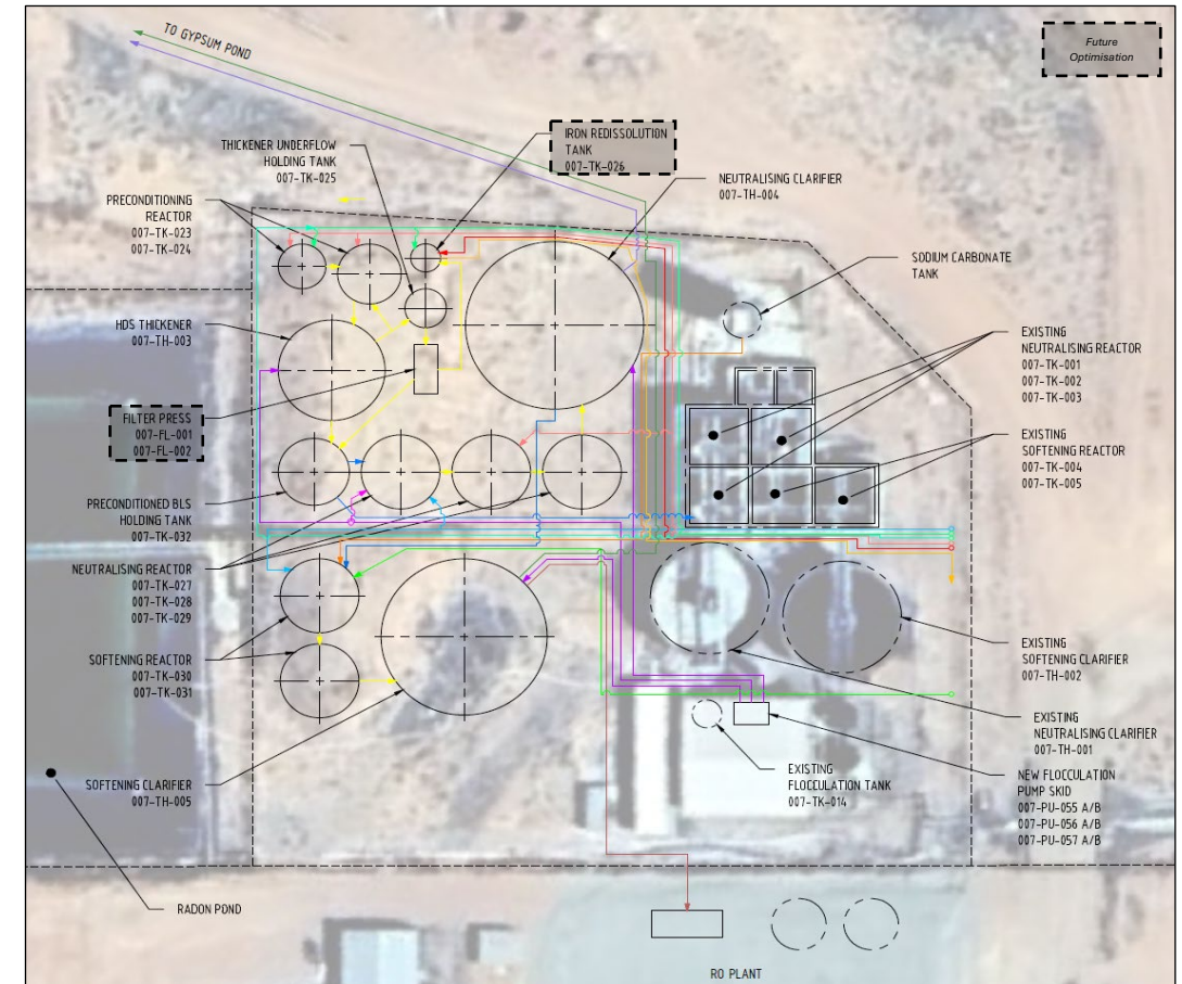
Indicative upgraded plant layout
