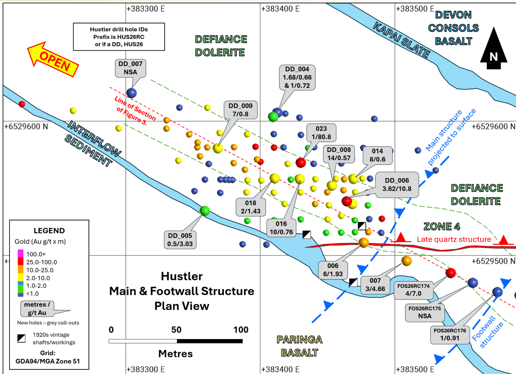
Figure 5: Plan view of Hustler illustrating recent results (large spheres), the Main and Footwall structures and key observed surface geological structures/features.
