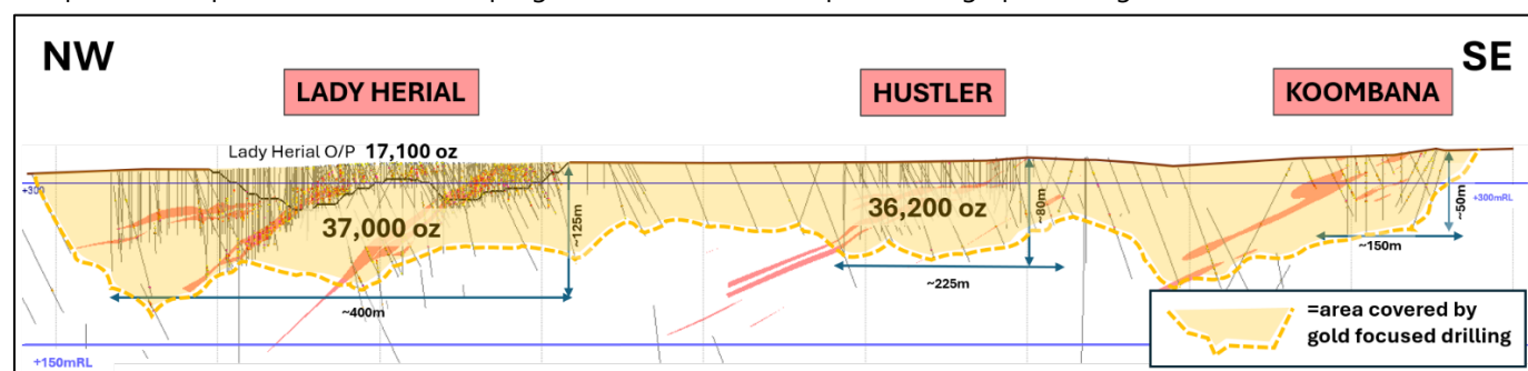
Figure 1: Diagrammatic long section looking north-east showing relative location of Hustler, Koombana and Lady Herial, with current MRE 3 gold ounces and the amount of gold that mining depleted from the last reported Lady Herial MRE (shown directly above the open pit outline).
