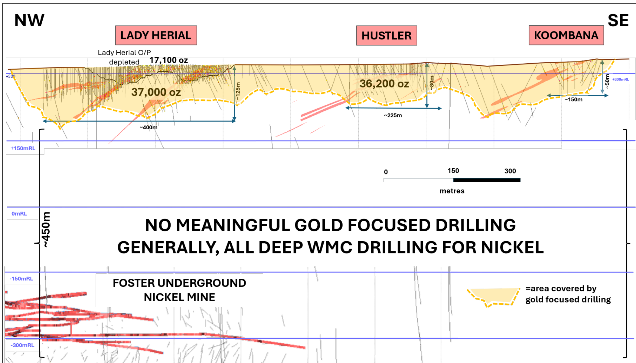
Figure 7: Long Section - Lady Herial on left and Koombana on right. Illustrating depth of current drill cover from surface with a gold focus, versus significant dip extent with no meaningful drill coverage. See page 17 for details of the gold MRE referenced.
