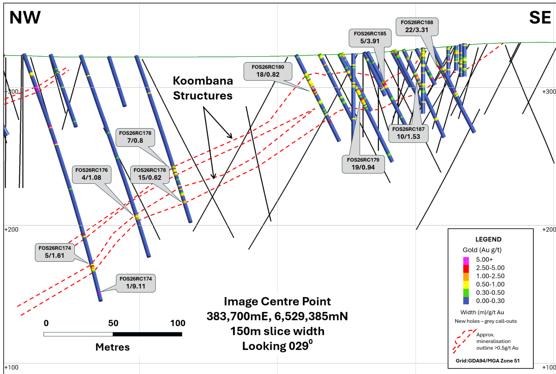
Figure 4: Sectional view of Koombana illustrating recent results.
