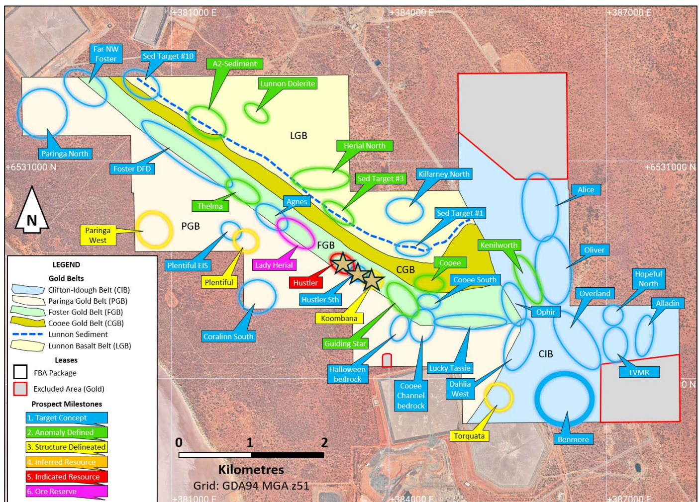
Figure 2: Plan view of the FBA project showing FY2027 drill targets and Koombana, Hustler and Lady Herial highlighted in the Foster Gold Belt.
