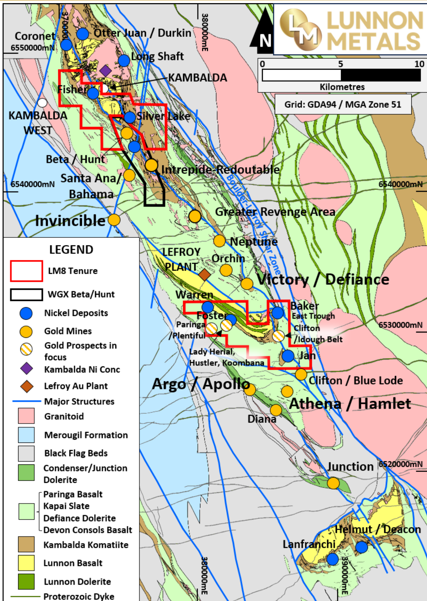
Figure 8: Location of the KGNP (red outlines) at the local Kambalda Nickel District / St Ives Gold Camp scale; showing surface geology and structure of this significant Australian gold camp.
