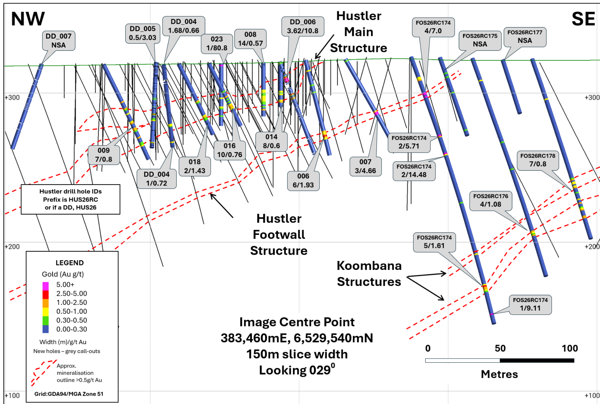
Figure 3: Sectional view of Hustler illustrating recent results, the Main and Footwall structures with Koombana plunging below both.
