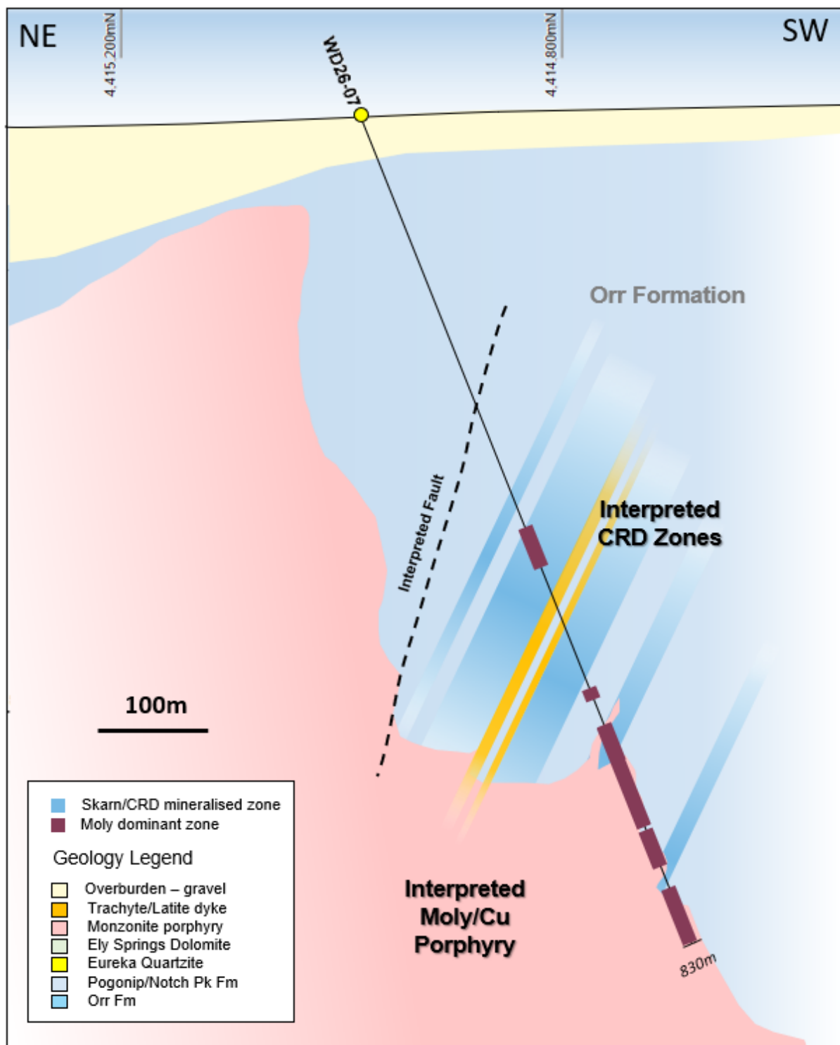
Figure 7: Schematic NE-SW geological section through drill hole WD26-07 (+/-100m) showing main geological units and drilling. A simplification of the mineralised intervals is shown.
