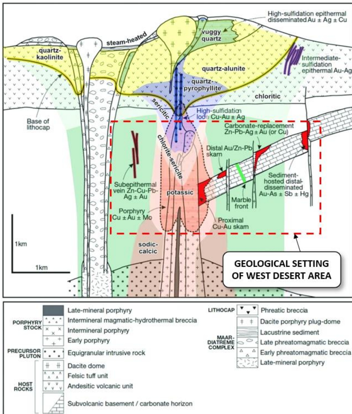
Figure 12: Schematic geological model of a typical porphyry mineralisation system (Sillitoe 2010) showing the approximate location and elements of the system West Desert area (red dotted outline).
