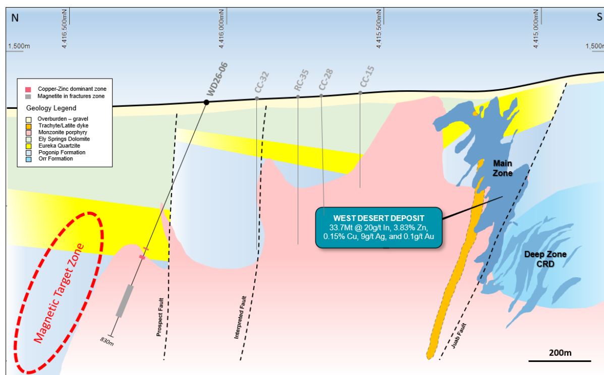
Figure 8: Schematic geological section at 289,025E (+/-200m) showing main geological units and WD26-06 drill trace.
