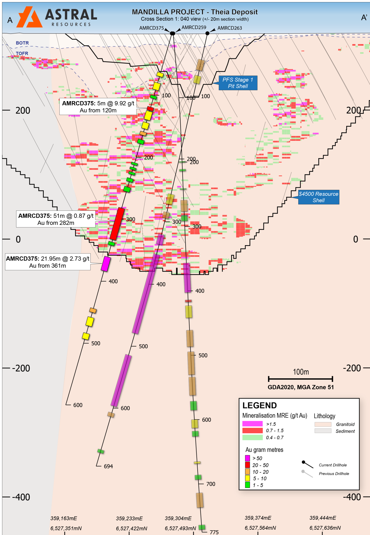
Figure 3 – Cross-section view of the Theia Deposit showing AMRCD375.
