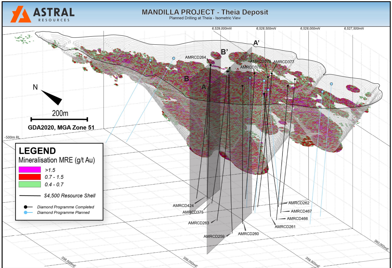
Figure 2 – Isometric view of the Theia Deposit showing the MRE block model, the drill traces for the completed and planned deep DD holes and the cross-section locations
