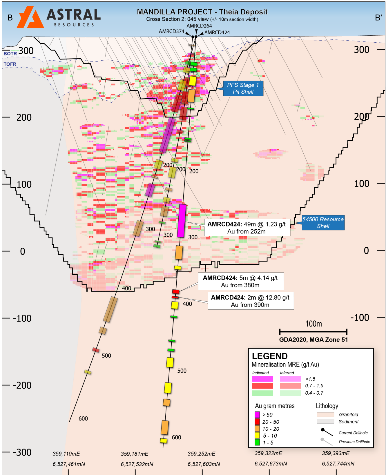
Figure 4 – Cross-section view of the Theia Deposit showing AMRCD424.
