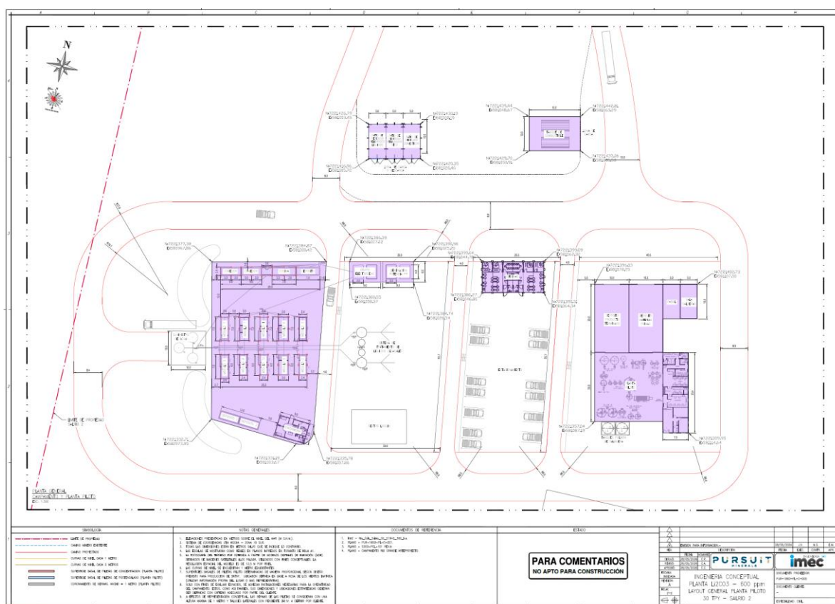
Figure 3 – Rio Grande Sur Pilot Plant Site Infrastructure Layout
