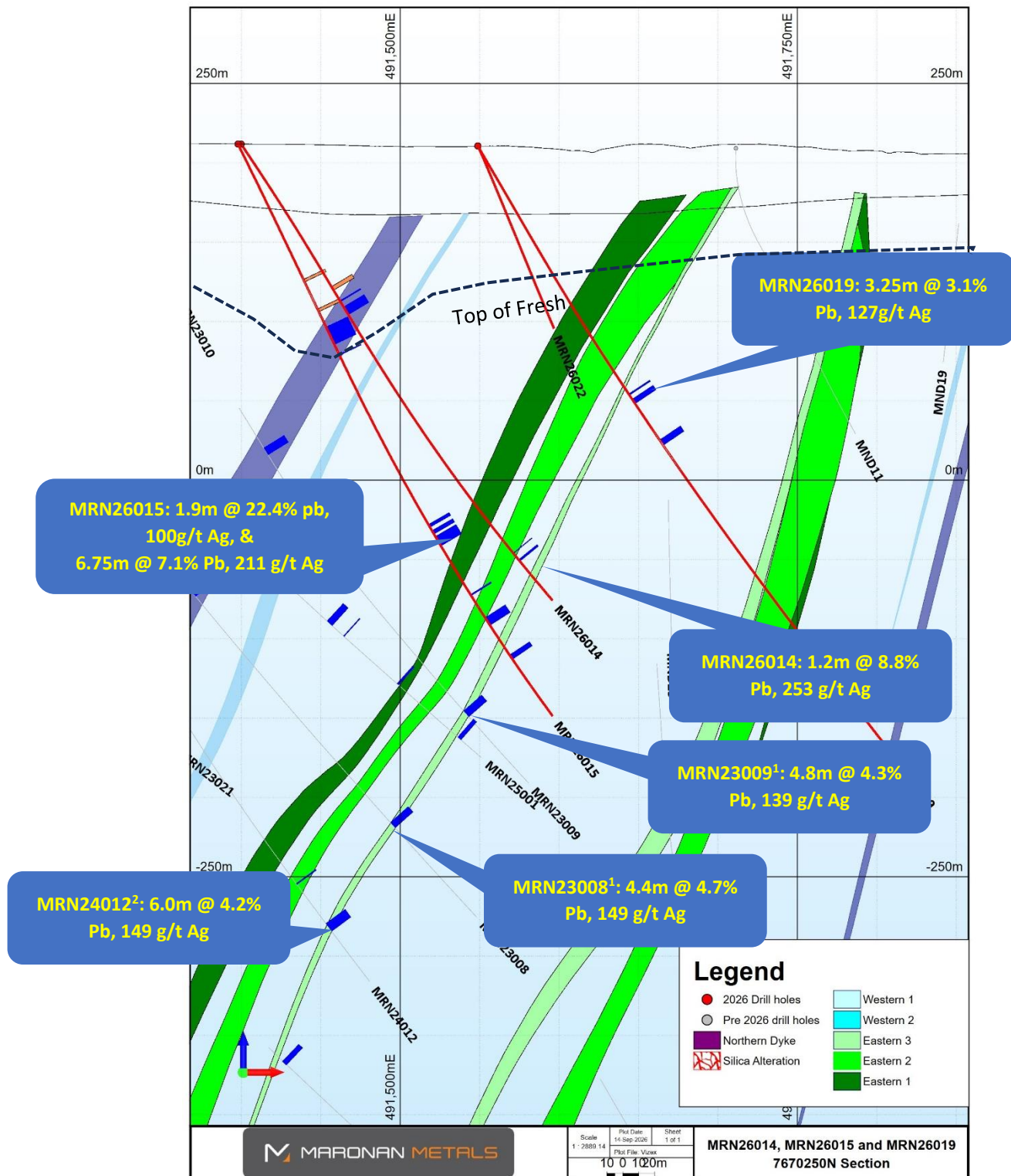
Figure 7: Section F – F' showing MRN26014, MRN26015 and MRN26019. 1 – 9/8/2023 – More High Tenor Silver with Lead in Shallow Starter Zone. 2 - 6/3/2025 – Drilling continues to deliver High Value Intercepts
