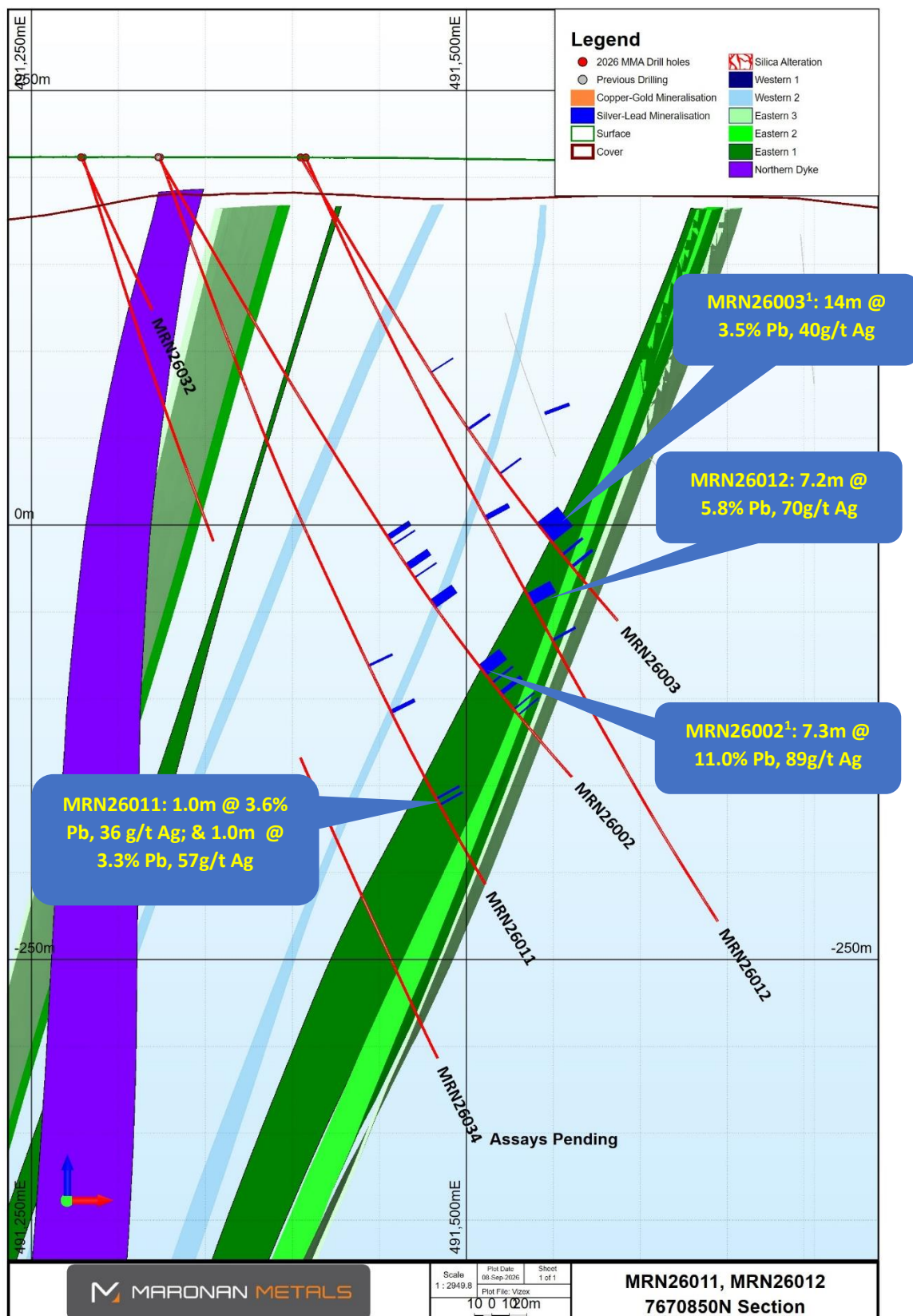
Figure 2: Section A – A' showing MRN26011 and MRN26012. 1 – 15/7/2026 – Drilling Intersects High Grade Silver Lead Mineralisation
