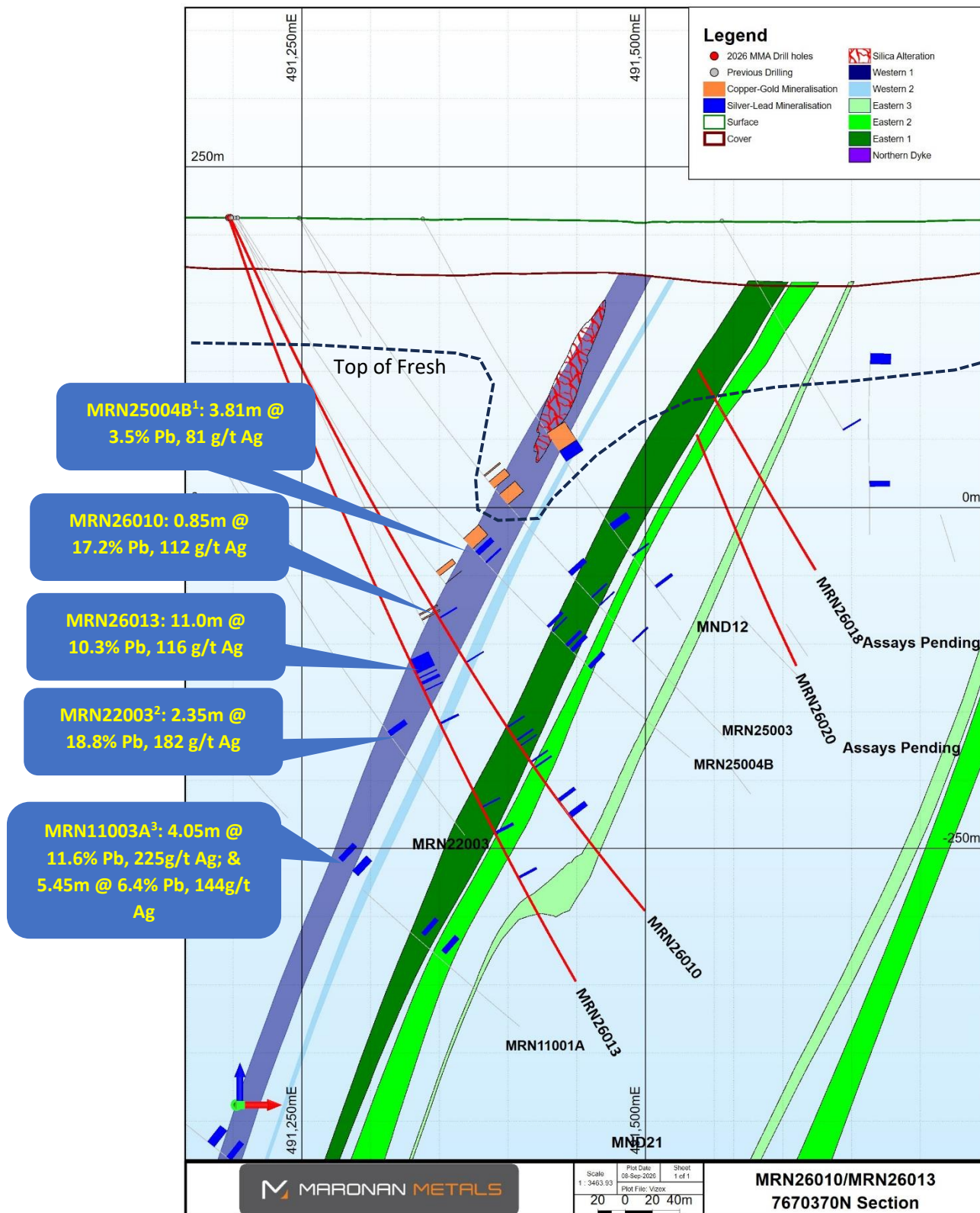
Figure 5: Section D – D' showing MRN26010 and MRN26013. 1- 15/5/2026 – Shallow Copper-Gold and Silver-Lead Drilling Results. 2- 16/1/2023 – Very High Grade Lead-Silver Assays in Shallower “Target 1” area. 3 - 27/4/2022 Maronan Metals Prospectus
