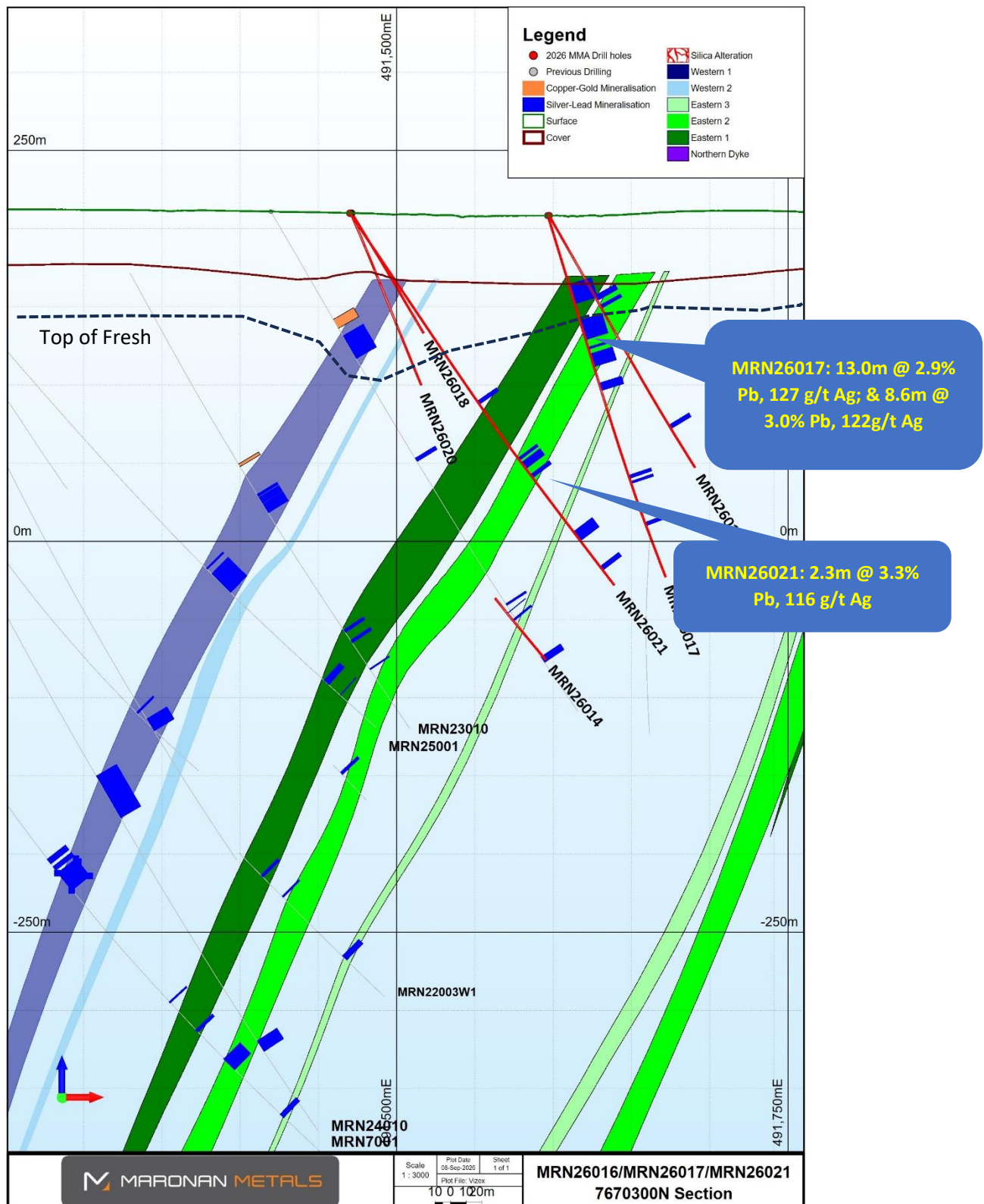
Figure 6: Section E – E' showing MRN26016, MRN26017 and MRN26021
