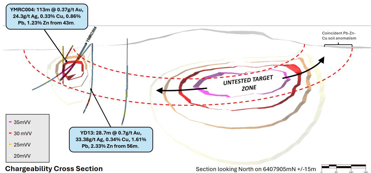
Figure 11: Yellow Mountain Chargeability Cross Section 14
