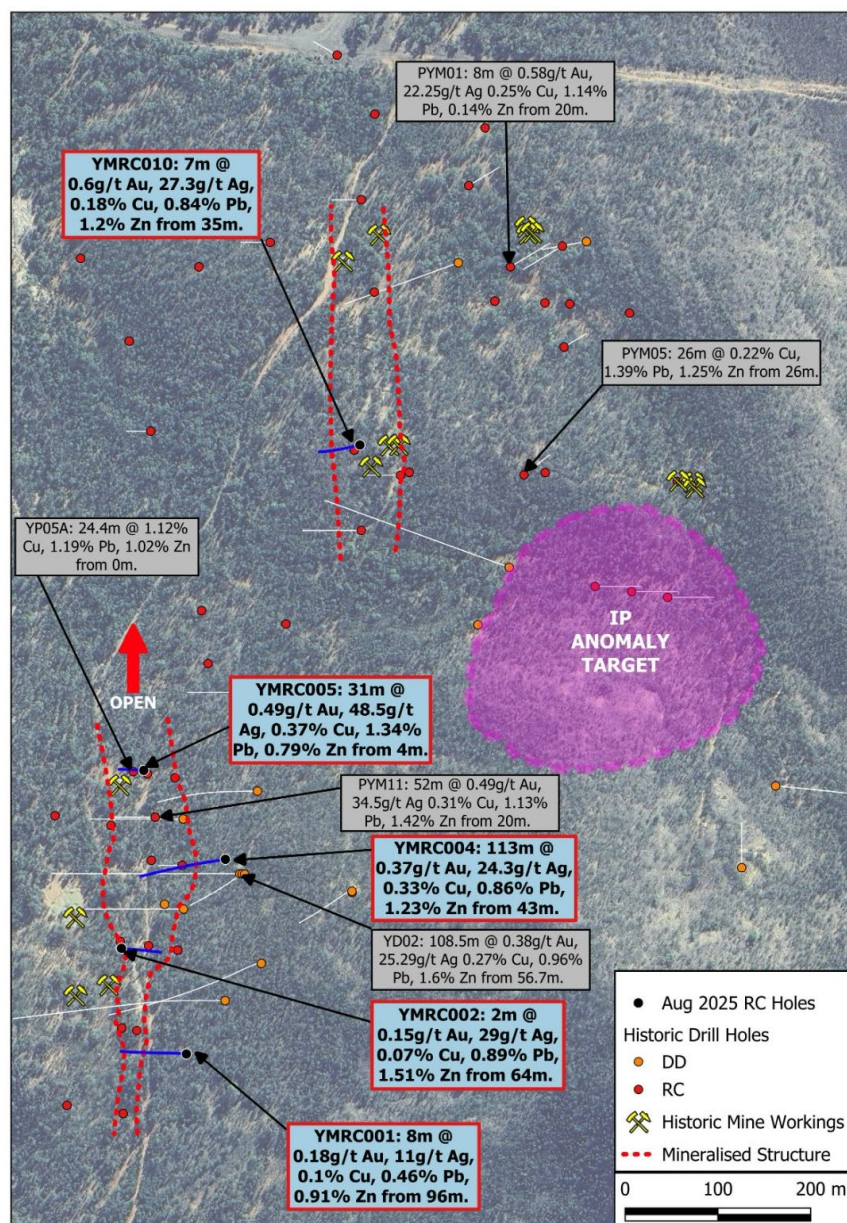
Figure 7: Yellow Mountain significant results from 2025 drill campaign (blue) 4,12
