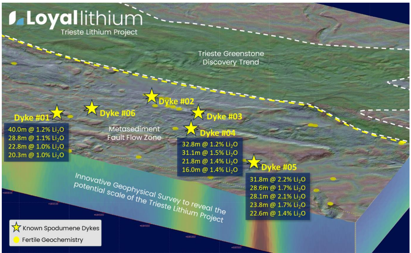
Figure 3: Trieste Lithium Project – Notable Drill intercepts displayed across a 3D Trieste landscape. (6, 7, 8)
