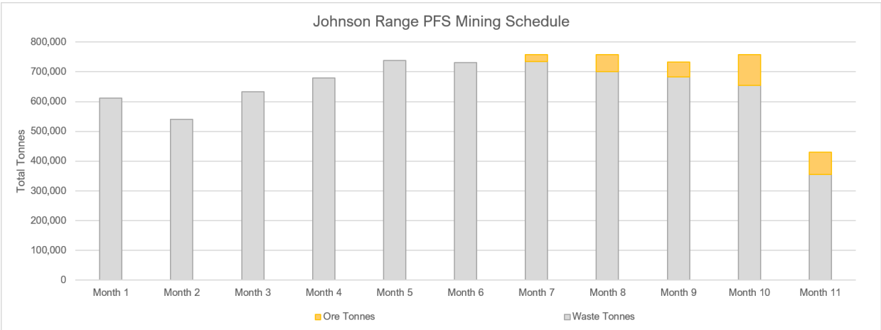
Figure 8: Johnson Range Mining Schedule
