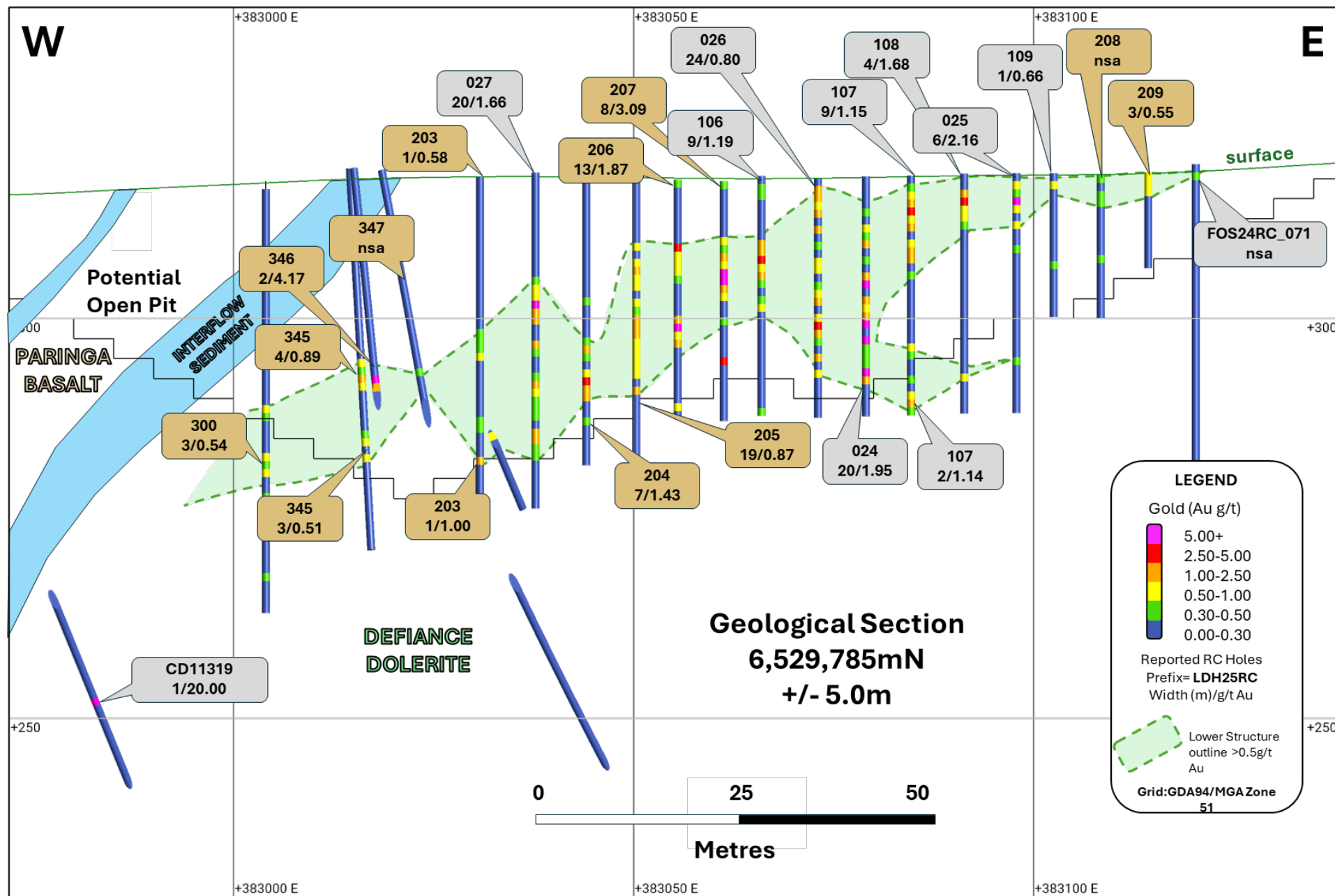
Figure 5: Section 6,529,785mN (looking north +/- 5m) illustrating the results reported today (gold call-outs) and prior reported results (grey call-outs).
