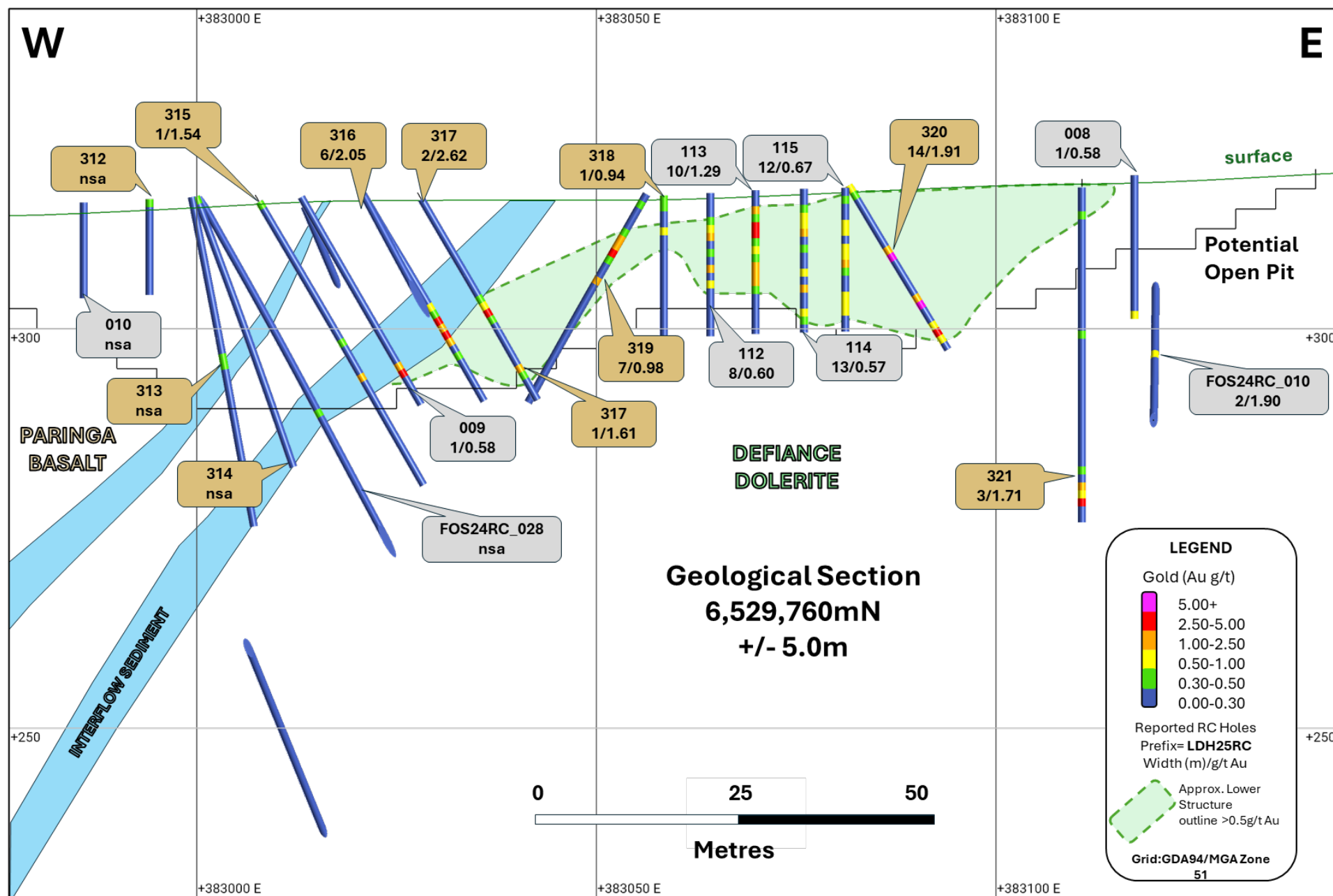
Figure 6: Section 6,529,760mN (looking north +/- 5m) illustrating the results reported today (gold call-outs) and prior reported results (grey call-outs).
