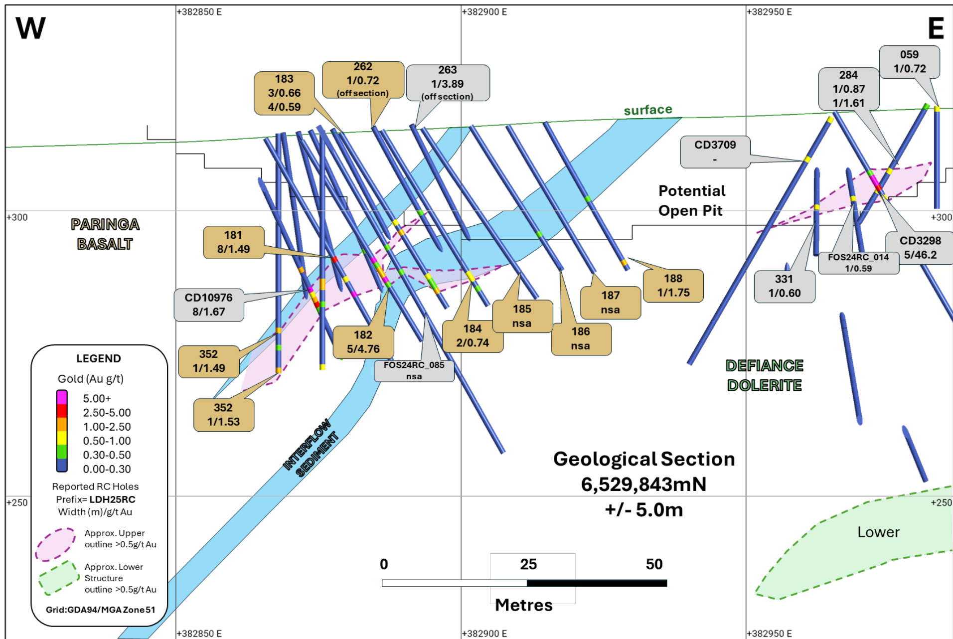
Figure 8: Section 6,529,843mN (looking north +/- 5m) illustrating the results reported today (gold call-outs) related to the sediment hosted Upper Structure and prior reported results (grey call-outs).
