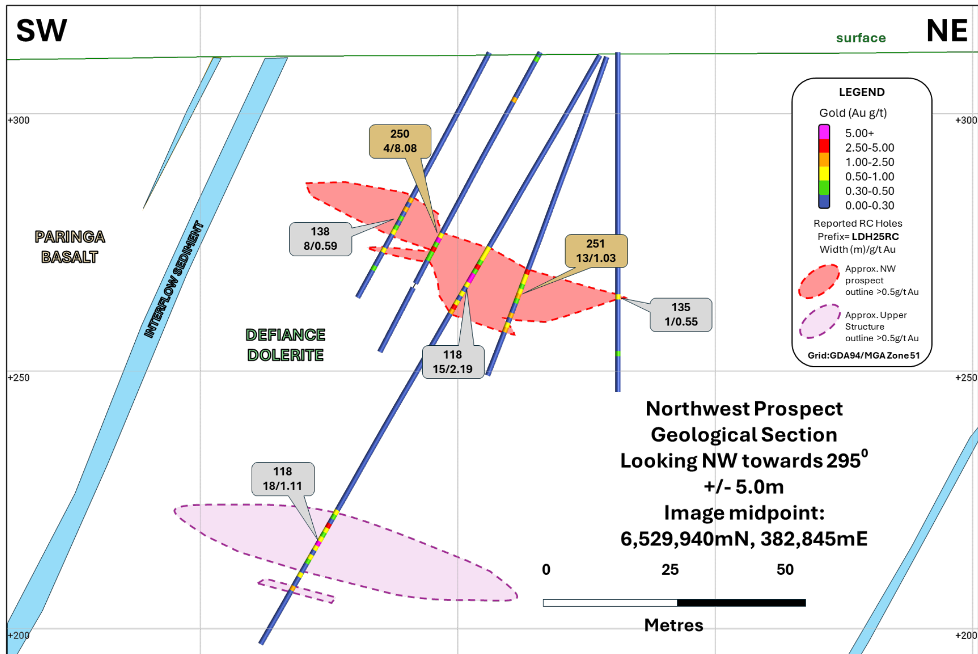
Figure 12: Section (looking northwest +/- 5m) illustrating the Northwest Prospect results reported today (gold call-outs) and prior reported results (grey call-outs).
