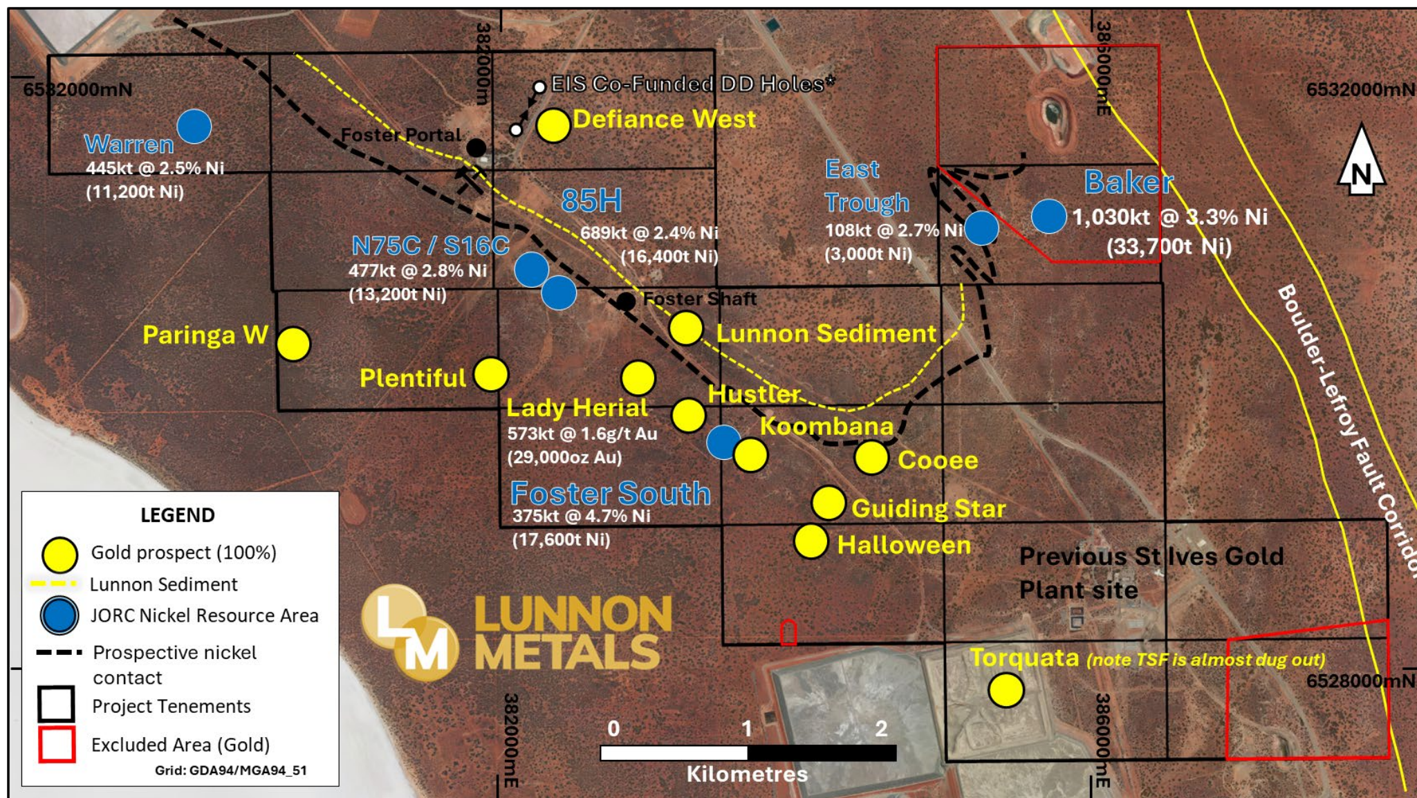
Figure 13: Foster-Baker Project Area showing select high-ranking gold prospects, gold & nickel Mineral Resource 5 positions.
