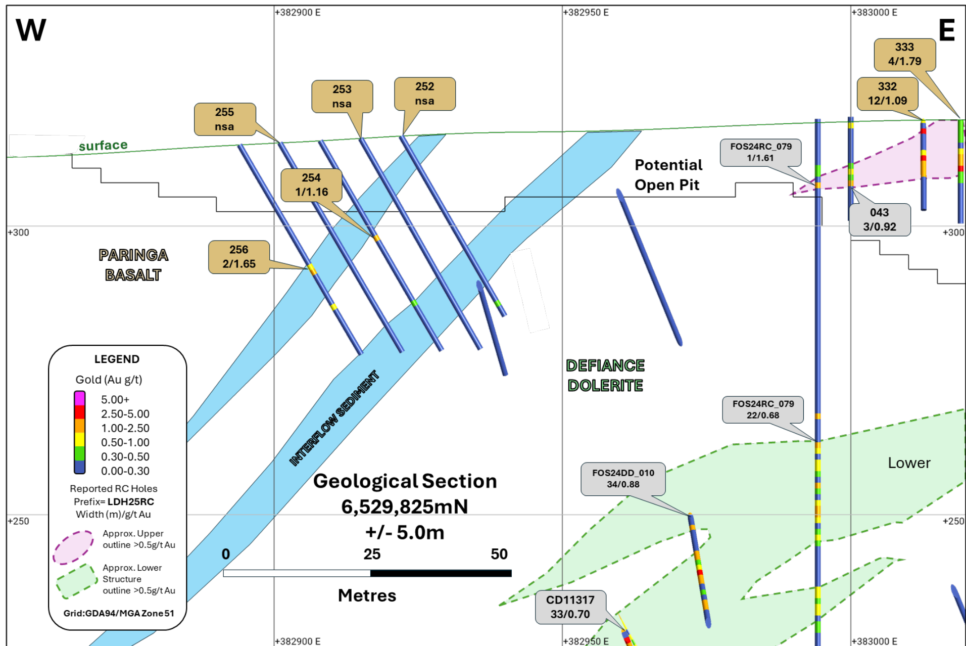
Figure 10: Section 6,529,825mN (looking north +/- 5m) illustrating the results reported today (gold call-outs) related to the sediment hosted Upper Structure and prior reported results (grey call-outs).
