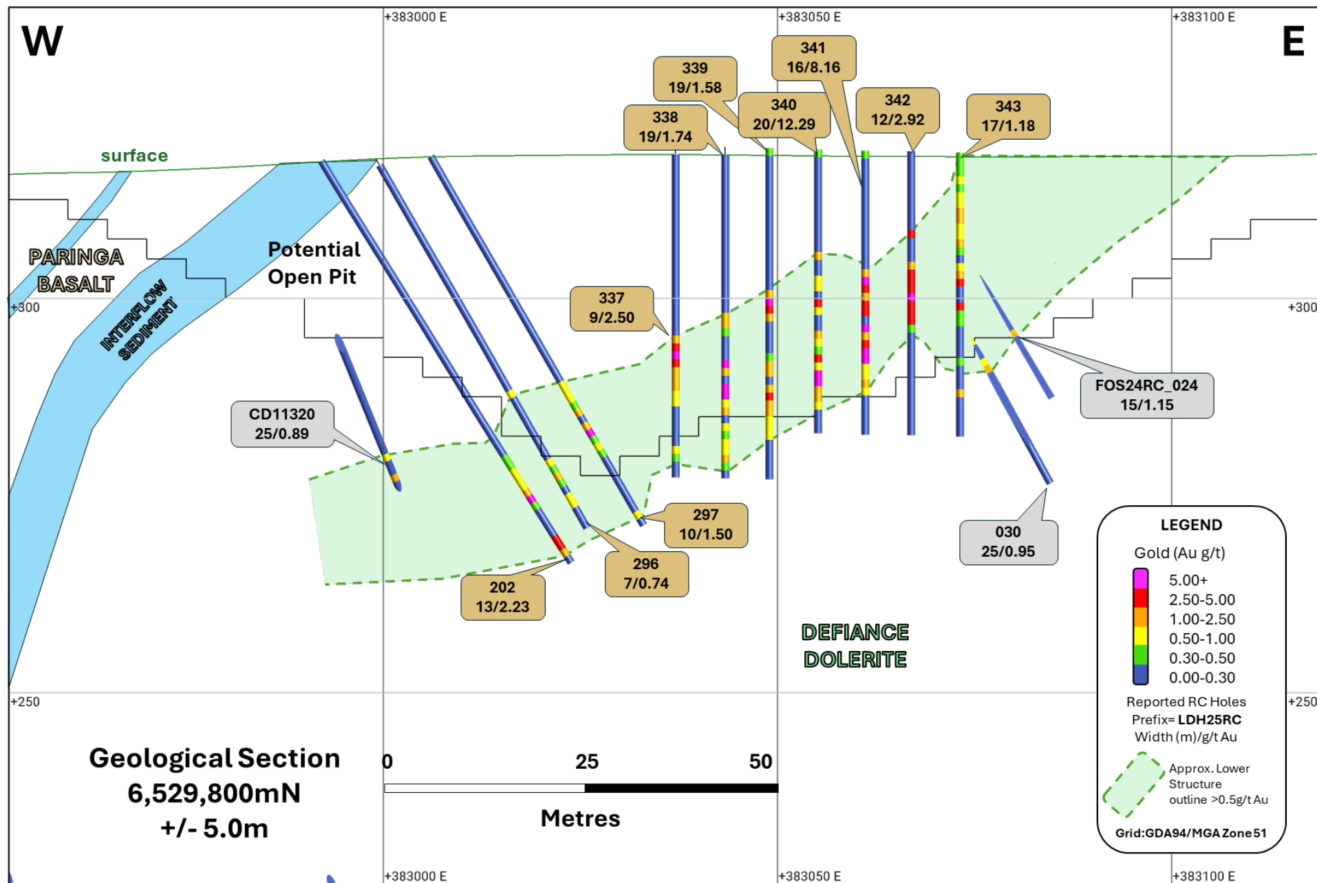
Figure 4: Section 6,529,800mN (looking north +/- 5m) illustrating the results reported today (gold call-outs) and prior reported results (grey call-outs).
