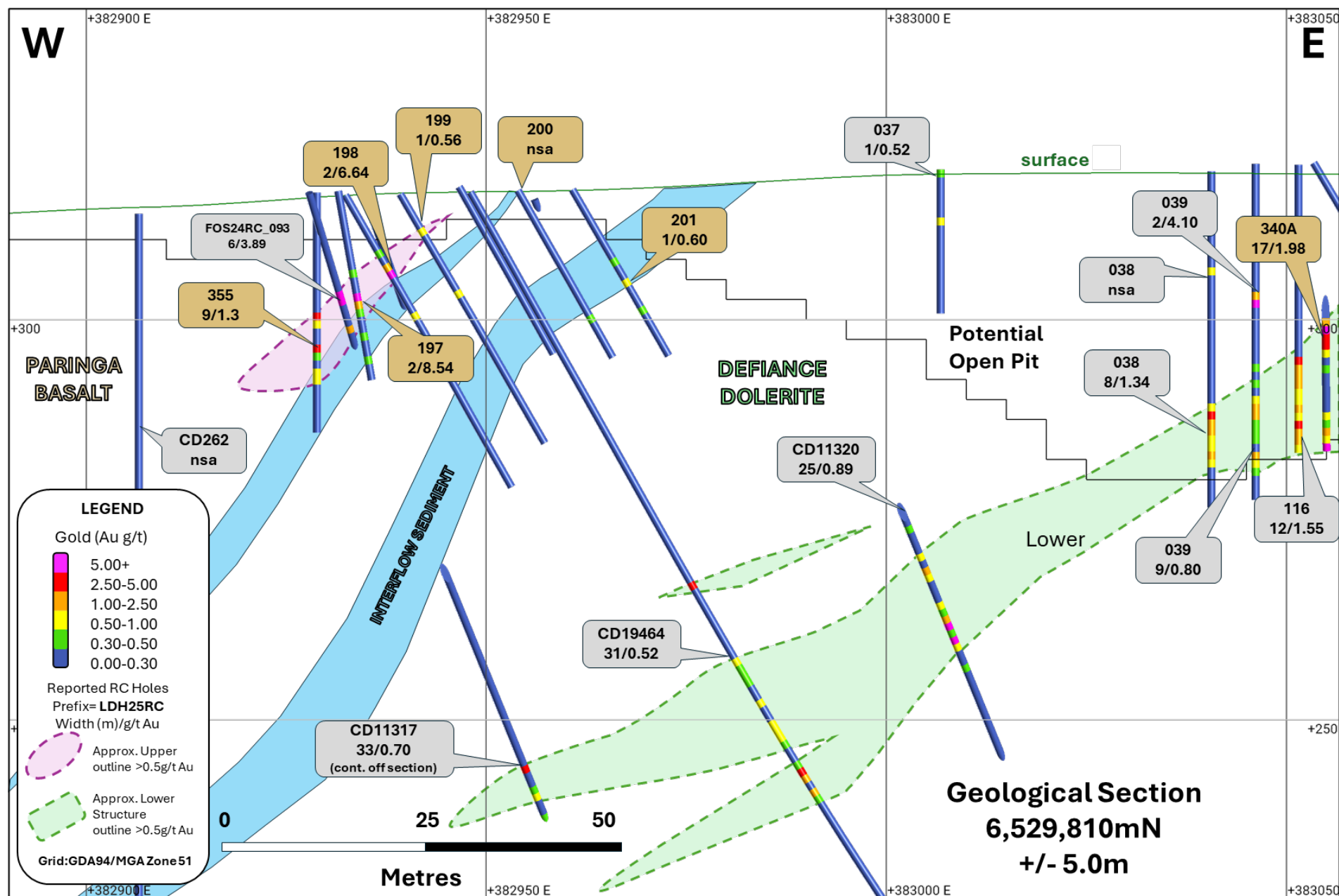
Figure 11: Section 6,529,810mN (looking north +/- 5m) illustrating the results reported today (gold call-outs) related to the sediment hosted Upper Structure and prior reported results (grey call-outs).
