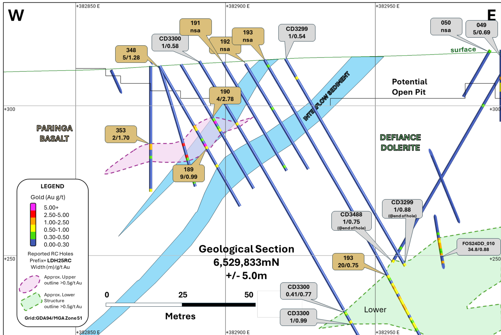
Figure 9: Section 6,529,833mN (looking north +/- 5m) illustrating the results reported today (gold call-outs) related to the sediment hosted Upper Structure and prior reported results (grey call-outs).
