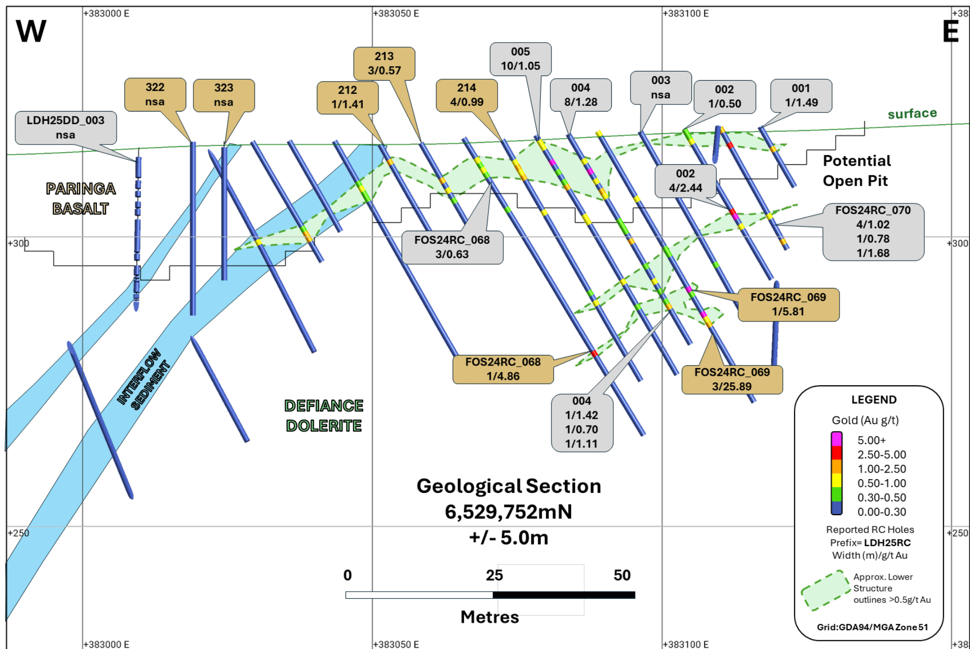
Figure 7: Section 6,529,752mN (looking north +/- 5m) illustrating the results reported today (gold call-outs) and prior reported results (grey call-outs).
