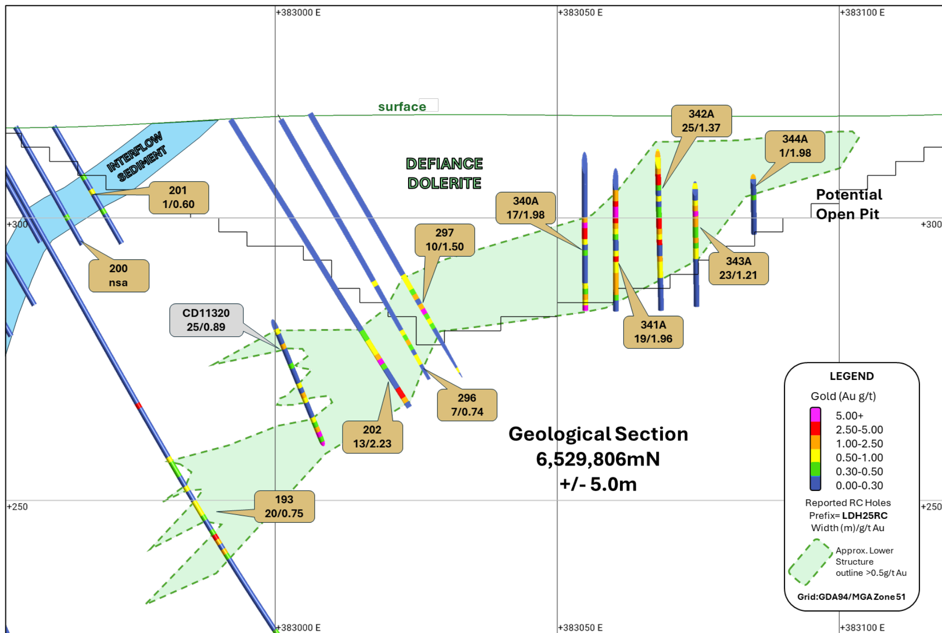
Figure 3: Section 6,529,806mN (looking north +/- 5m) illustrating the results reported today (gold call-outs) and prior reported results (grey call-outs).
