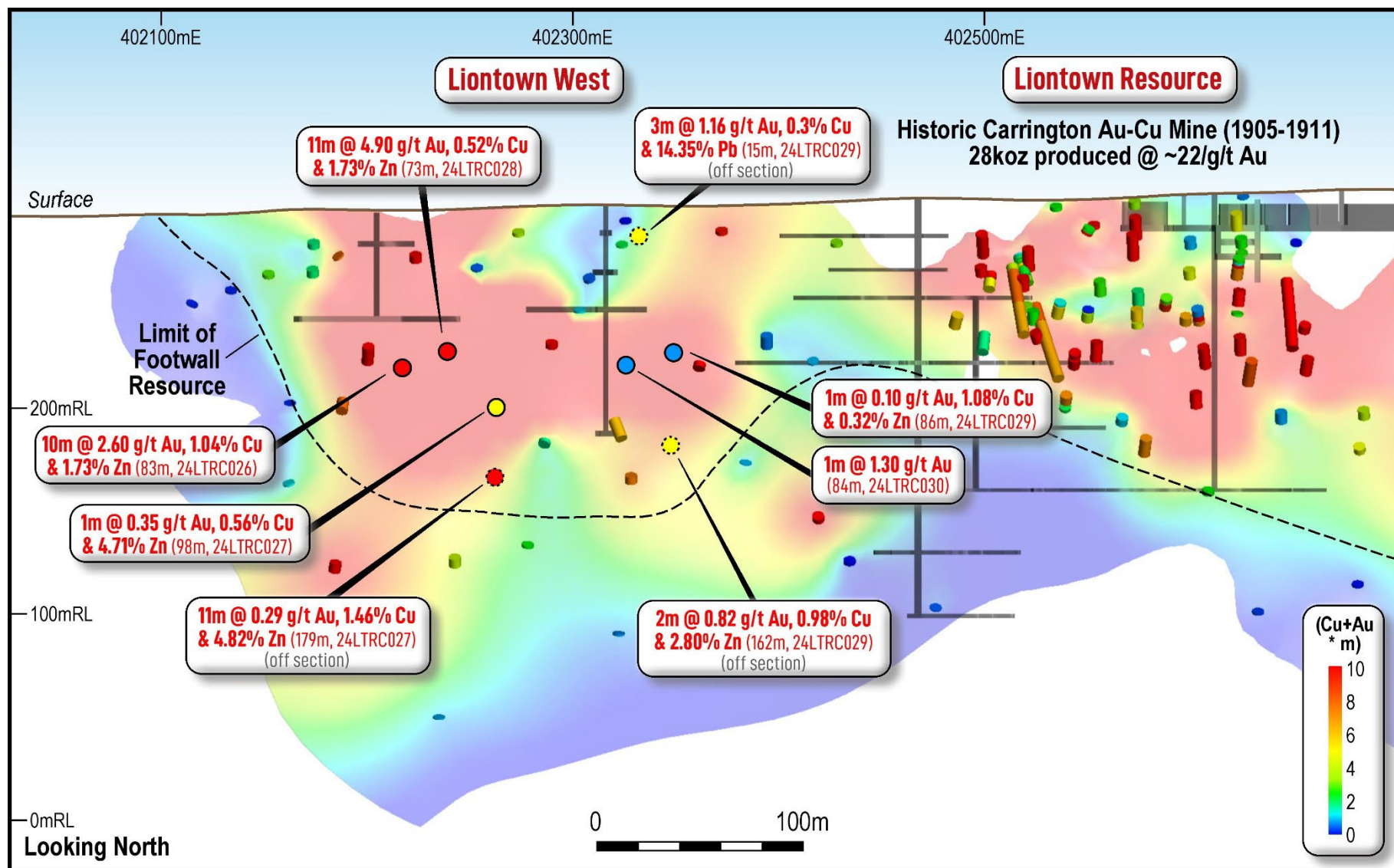
Figure 3: Long section (20m thick) of the Au-Cu rich footwall horizon at Liontown West, coloured by thickness. Historic workings including the Carrington Au-Cu Mine and completed infill RC holes are displayed.
