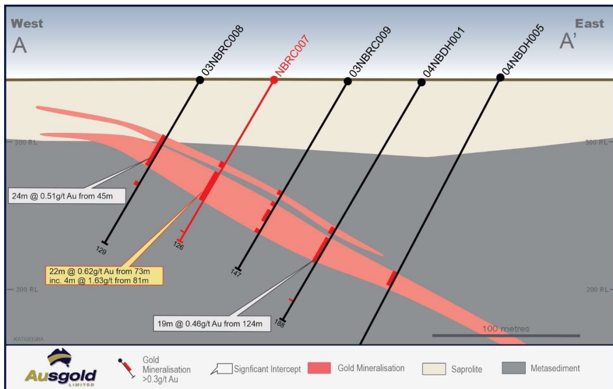
Figure 11 - Nanicup Bridge cross-section (A-A').
