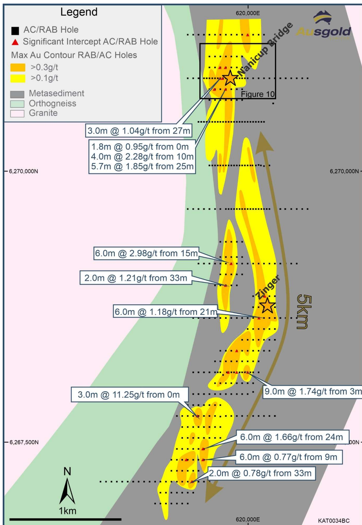
Figure 9 – Geology and mineralisation map of the Nanicut Bridge and Zinger Prospects.
