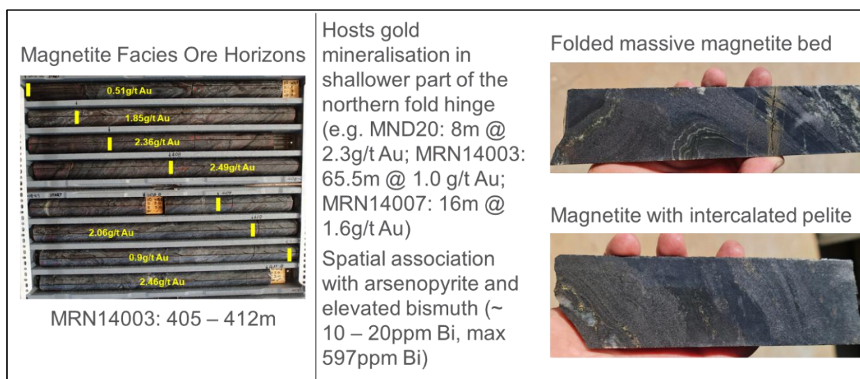
Figure 15: Example of gold only mineralisation hosted by magnetite BIF.
