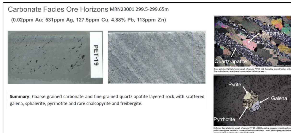
Figure 8: Petrographic thin section images and description of calcite type silver-lead mineralisation
