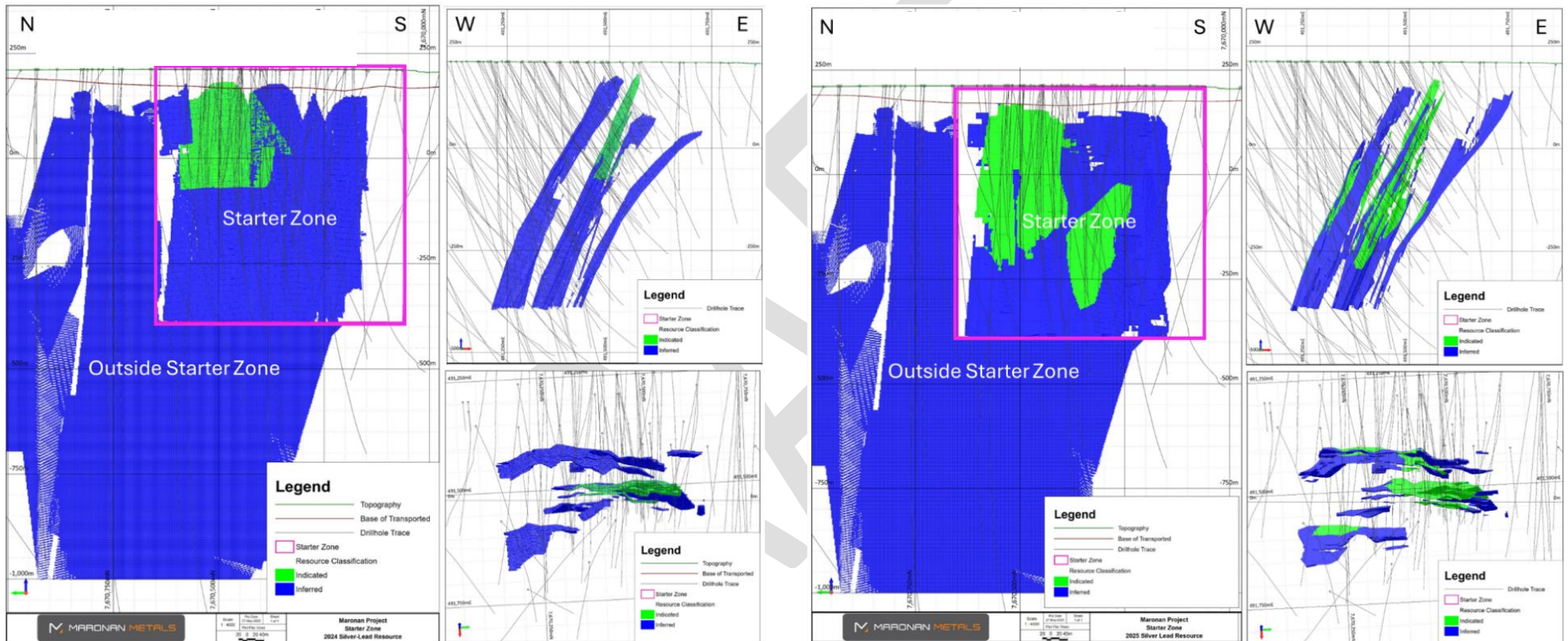
Figure 19: Maronan Project: Comparison between the 2024 and 2025 Silver Lead Resource Models coloured by resource classification (green = indicated, blue =inferred). The blocks are shown above the reported cut-off grade of >3% Lead. Long section view (left), section view (top right) and plan view (bottom right)
