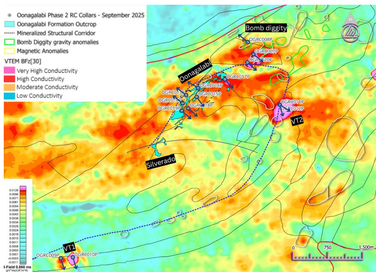
Figure 4. Oonagalabi VTEM BFz30 conductivity image showing the Priority 1 conductors, preliminary anomaly picks, interpreted prospective horizon, historic drillholes and proposed Phase 2 RC holes.
