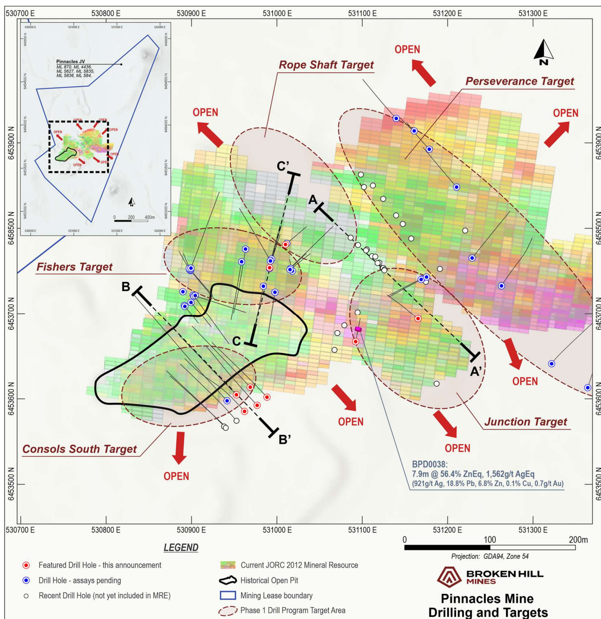
Figure 1 – Pinnacles Mine plan view showing BHM's phase 1 FY26 drilling target areas
