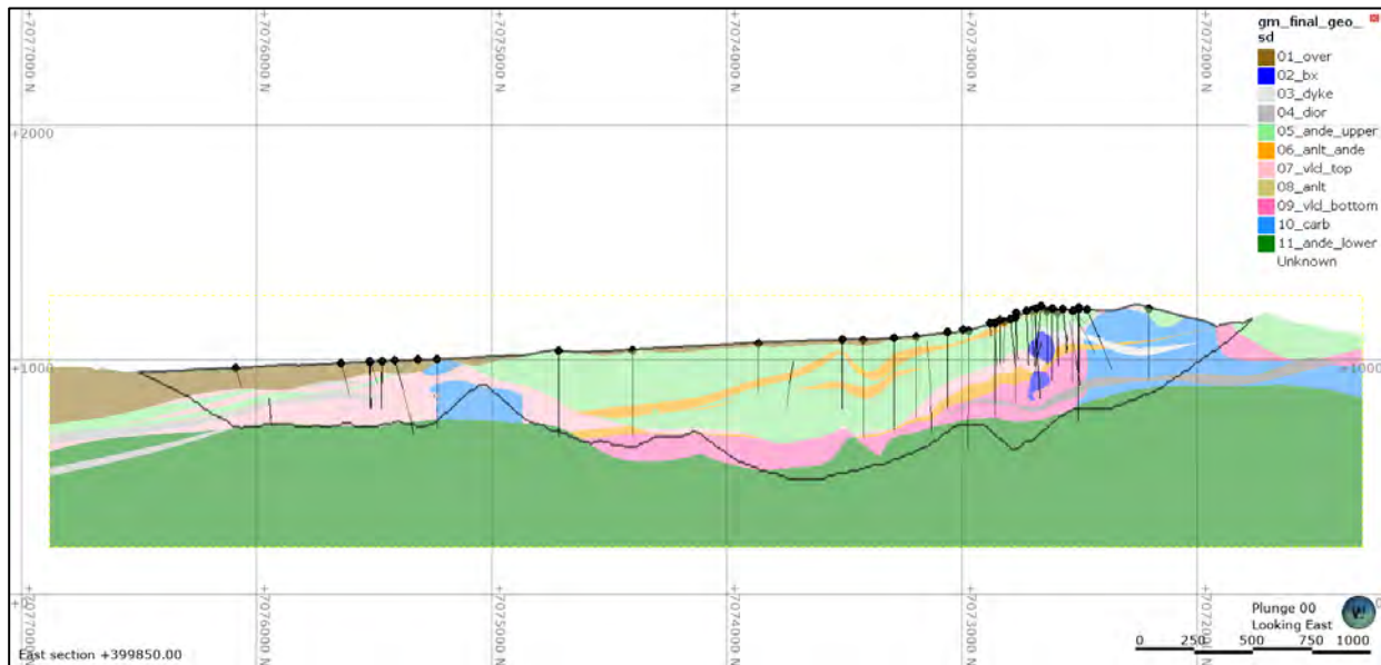
Figure 14-5: SD and IN Geology: Section 399,850E Looking East
