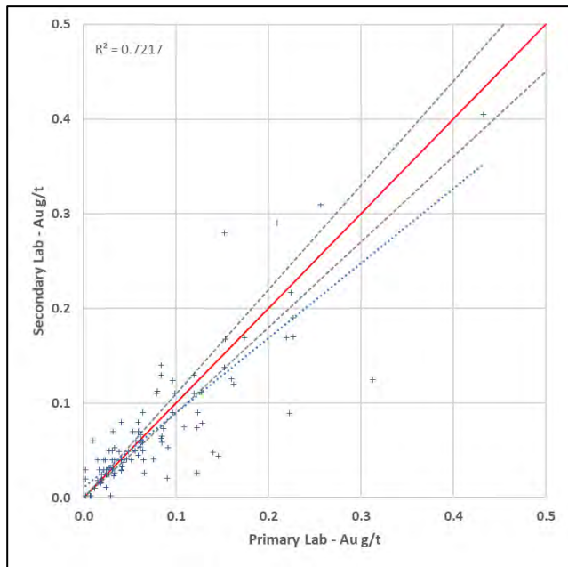
Figure 11-18: Check Assay Performance: Gold with \pm 10\% Guidelines
