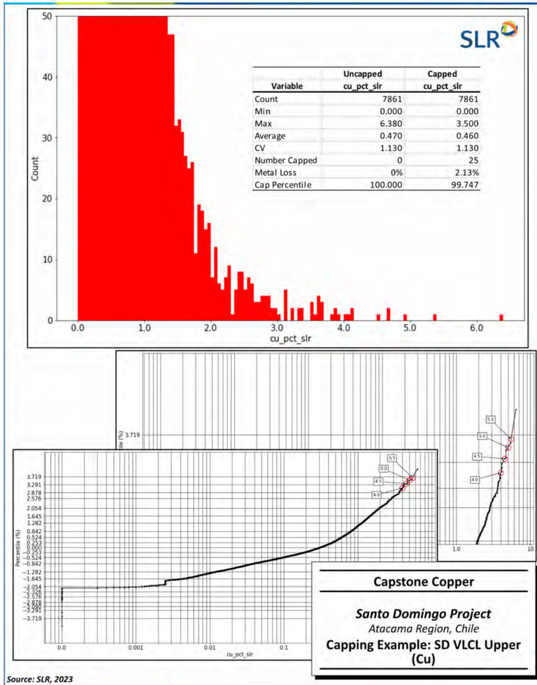
Figure 14-12: Capping Example: SD VLCL Upper (Cu)
