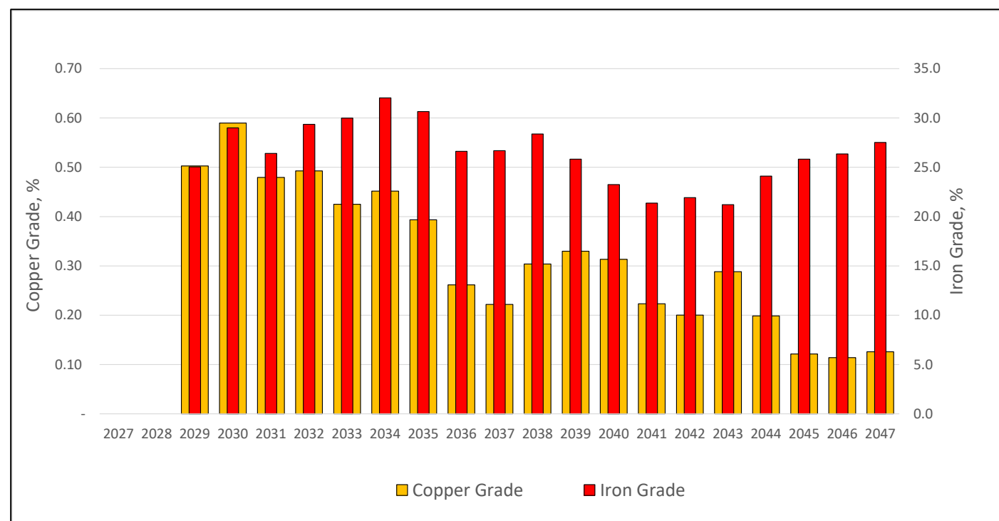
Figure 17-2: Iron and Copper Grade of Plant Feed
