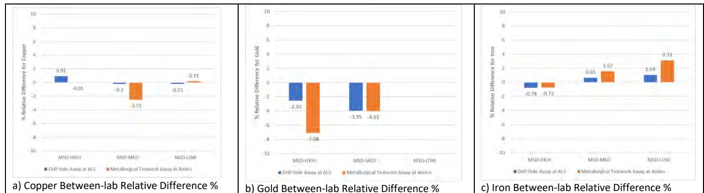
Figure 11-21: Bias between the Drill Hole Assay Dataset and Metallurgical Test Work Dataset within \pm 10\%
