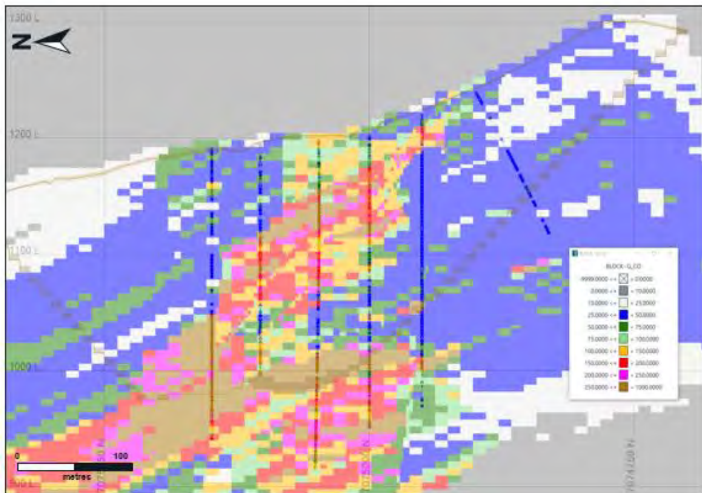
Figure 14-45: ES Visual Validation Example: Co Section 396,195E
