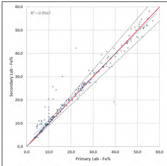
Figure 11-19: Check Assay Performance: Iron with \pm 10\% Guidelines
