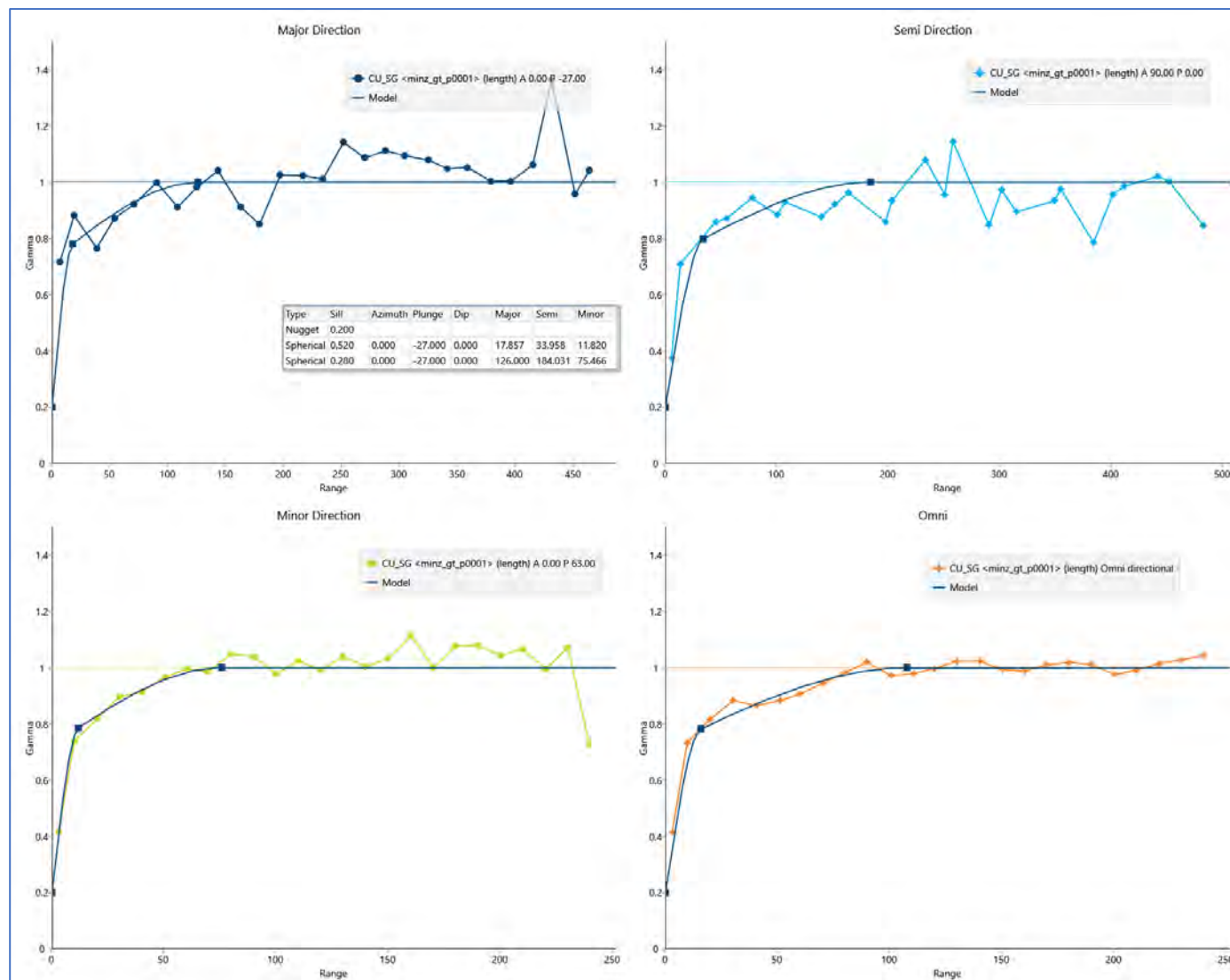
Figure 14-36: ES Variogram Example: Cu Accumulations
