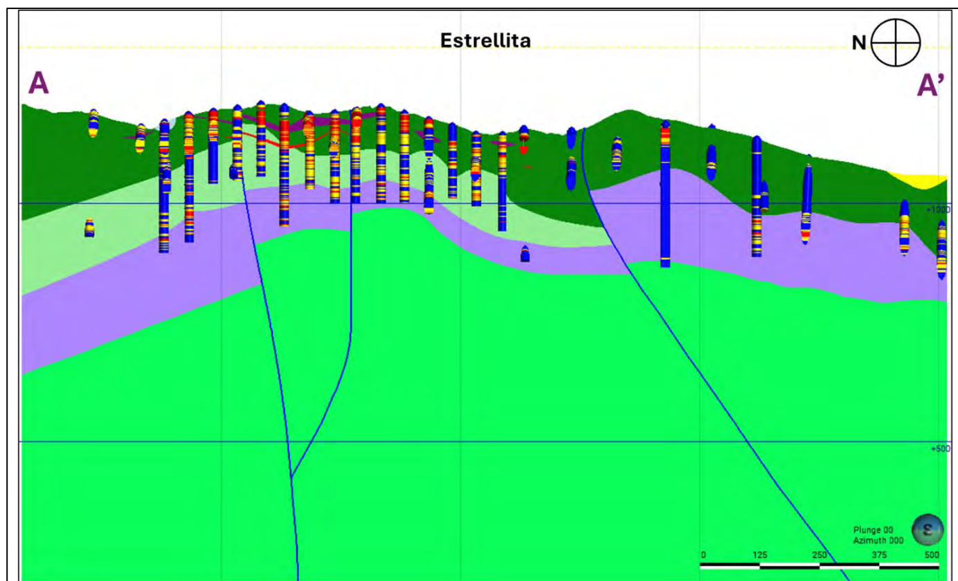
Figure 7-9: Simplified Geological Cross-Section, Estrellita
