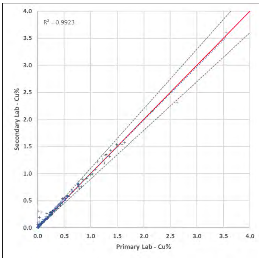
Figure 11-17: Check Assay Performance: Copper with \pm 10\% Guidelines
