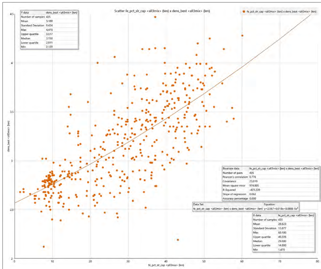
Figure 13-2: Density Regression Curve for Mixed Material: SD + IN
