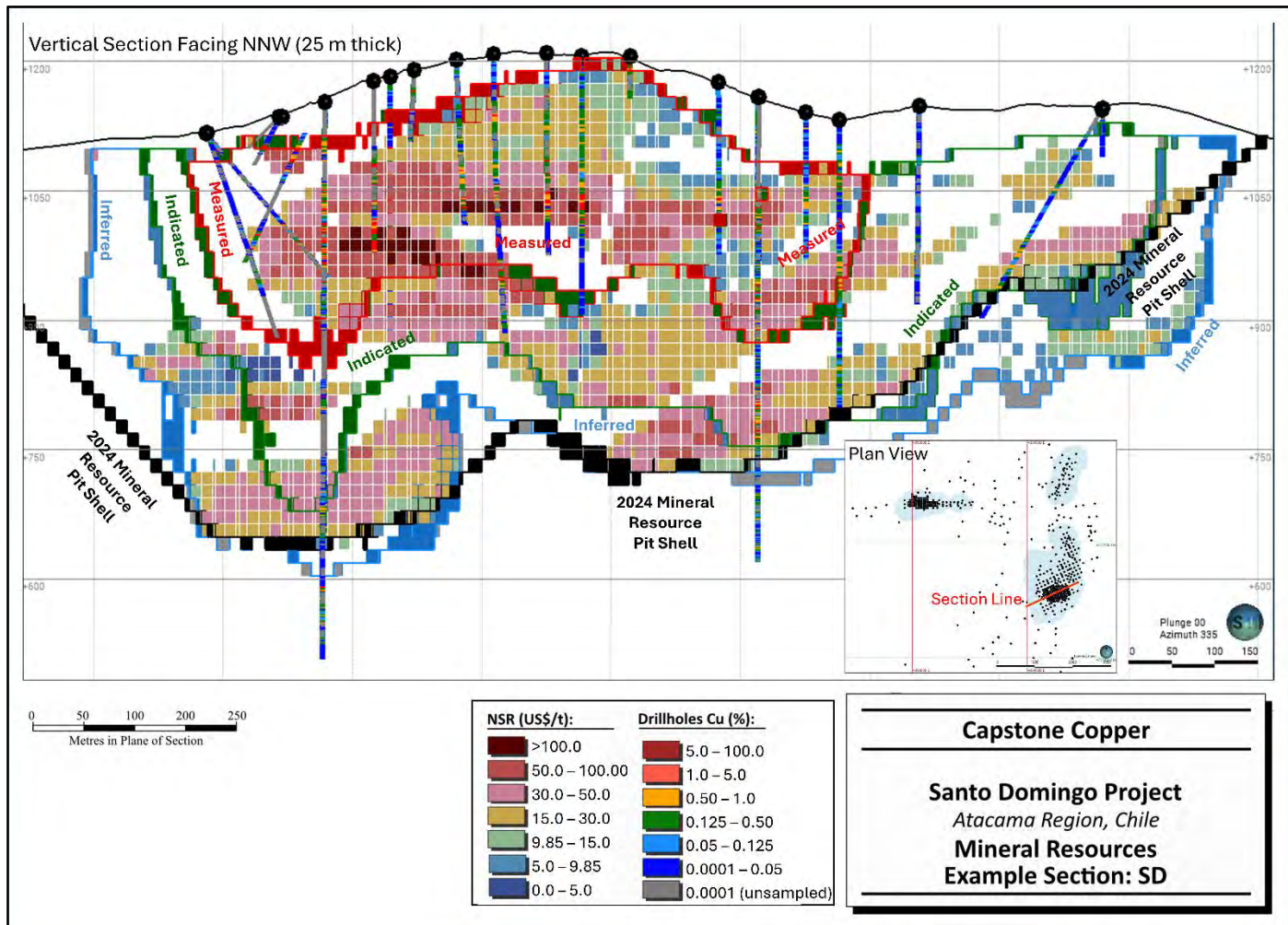
Figure 14-26: Example Mineral Resource Cross Section: SD
