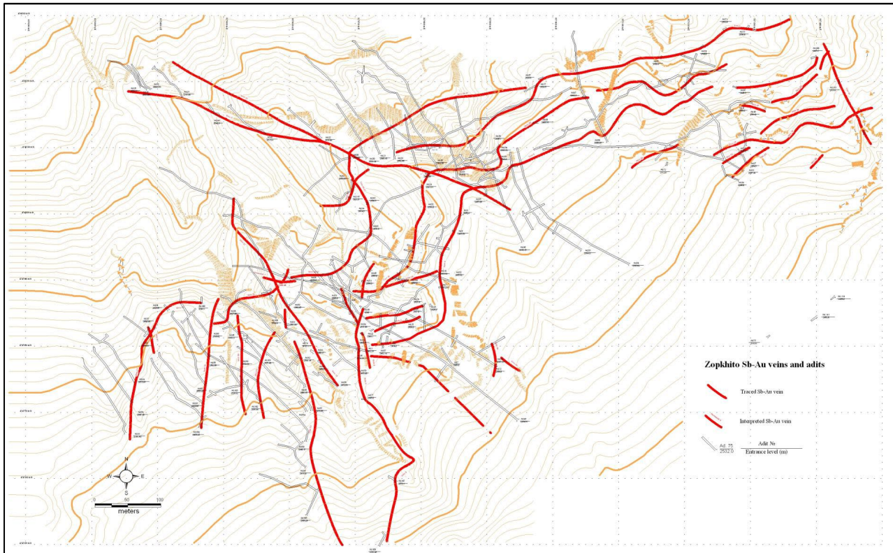
Figure 3 Map of Zopkhito veins and adits (EMED Mining report 2008)
