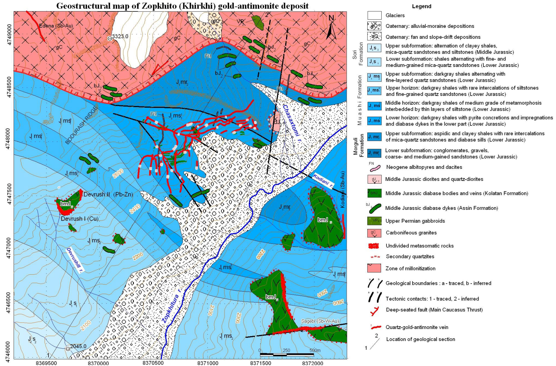
Figure 7 Geostructural map of Zopkhito Sb-Au deposit (from EMED 2008 report)
