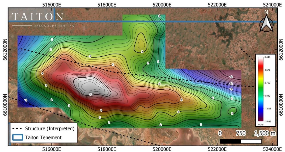
Figure 4. Yogi residual Bouguer gravity anomaly image over subset inversion model target area.
