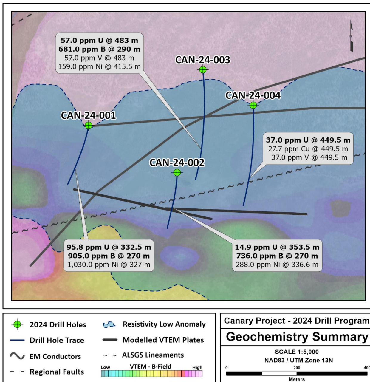
Figure 3 Map of the northern Canary conductor trend highlighting 2024 drill holes with 2008 VTEM in the background. The geophysical target area is defined by a significant resistivity low anomaly coinciding with EM conductors dipping to the north.
