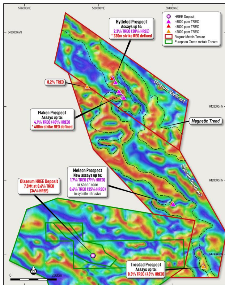
Figure 3: Airborne Magnetic Map (tilt derivative) showing the location of recent rock sample results (*TREO includes all rare earth elements plus Y and Sc)
