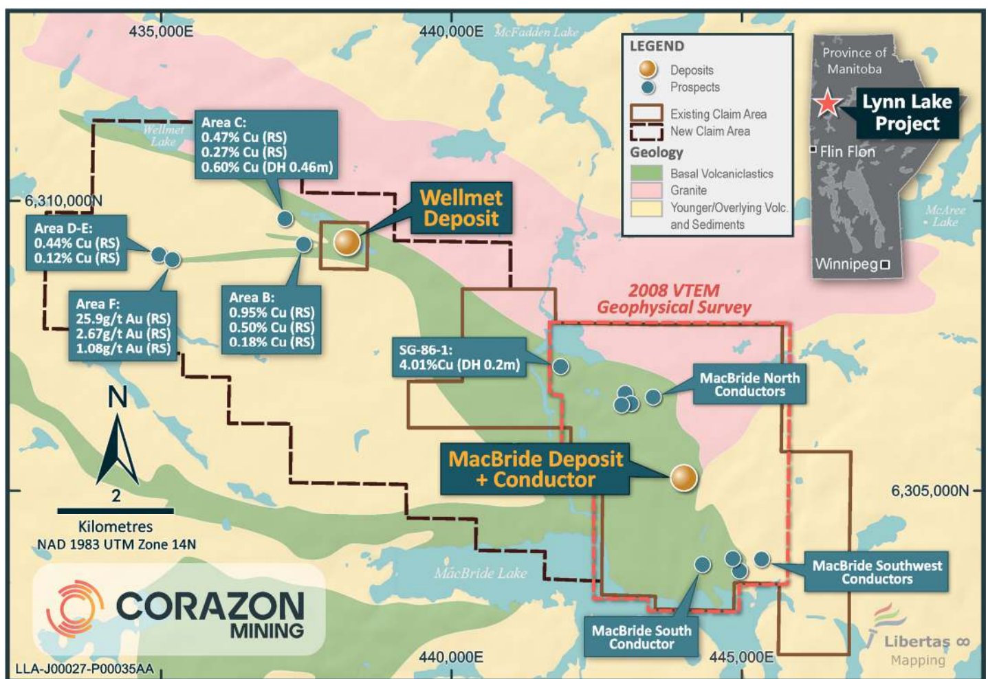
Figure 1 - Interpreted Geology of the MacBride Project, New Claim and 2008 VTEM area outlines, historically defined deposit and prospect locations. Geology modified from the Manitoba Geological Survey's 1:50,000 Mapsheet – Fraser Lake (64B13, GP87-3-3) 1993. Government provided selected sampling results defining the prospects include rock samples (RS = grab and channel samples) and drill samples (DH with sample interval in metres) as defined in digital datasets provided by the Manitoba Department of Economic Development, Investment, Trade and Natural Resources. Original source references for sampling and drilling results are provided within Table 1 of this report.
